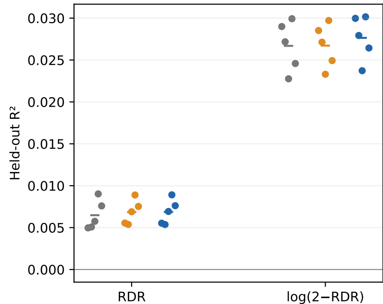
P vs Q_I
