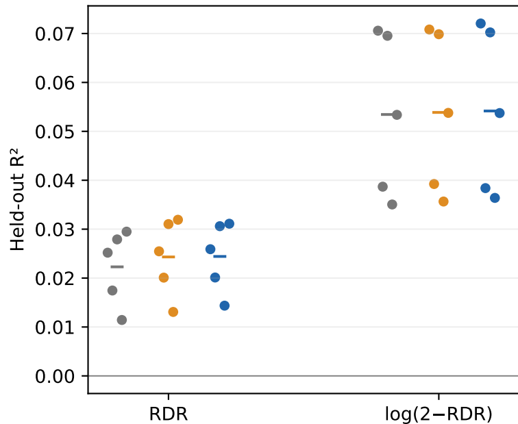
P vs Q_u
