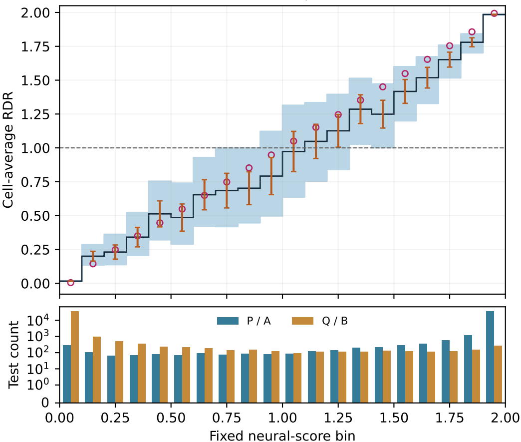
CelebA feature: merged held-out test, repeat 02 Nominal 95% cell-average intervals; same test pool for both estimates
