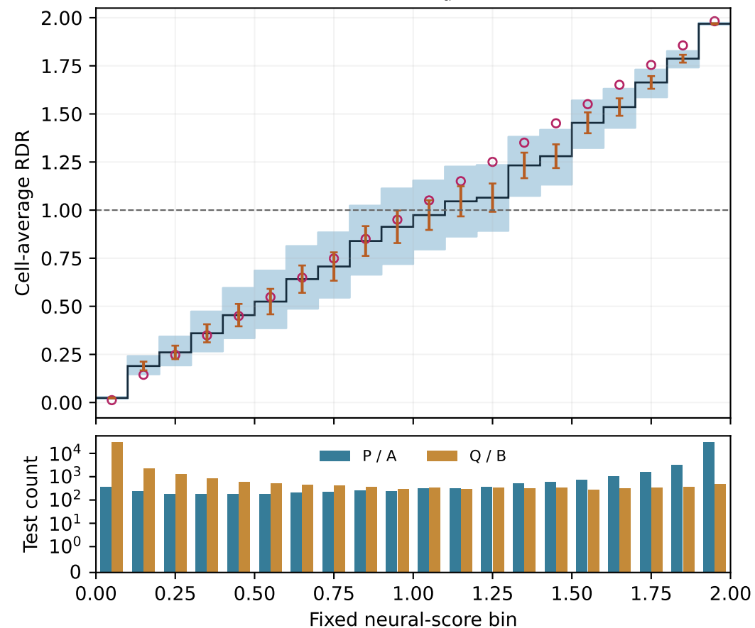
CelebA feature: merged held-out test, repeat 02 Nominal 95% cell-average intervals; same test pool for both estimates
