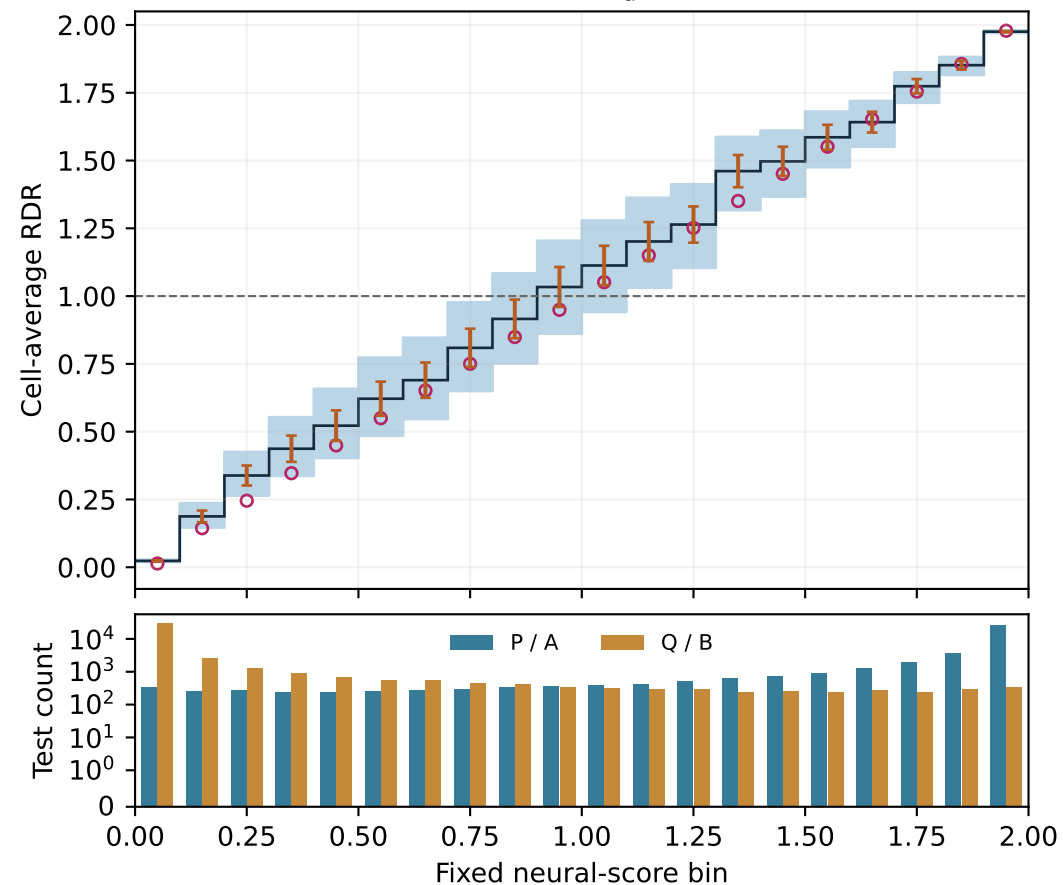
CelebA feature: merged held-out test, repeat 04 Nominal 95% cell-average intervals; same test pool for both estimates
