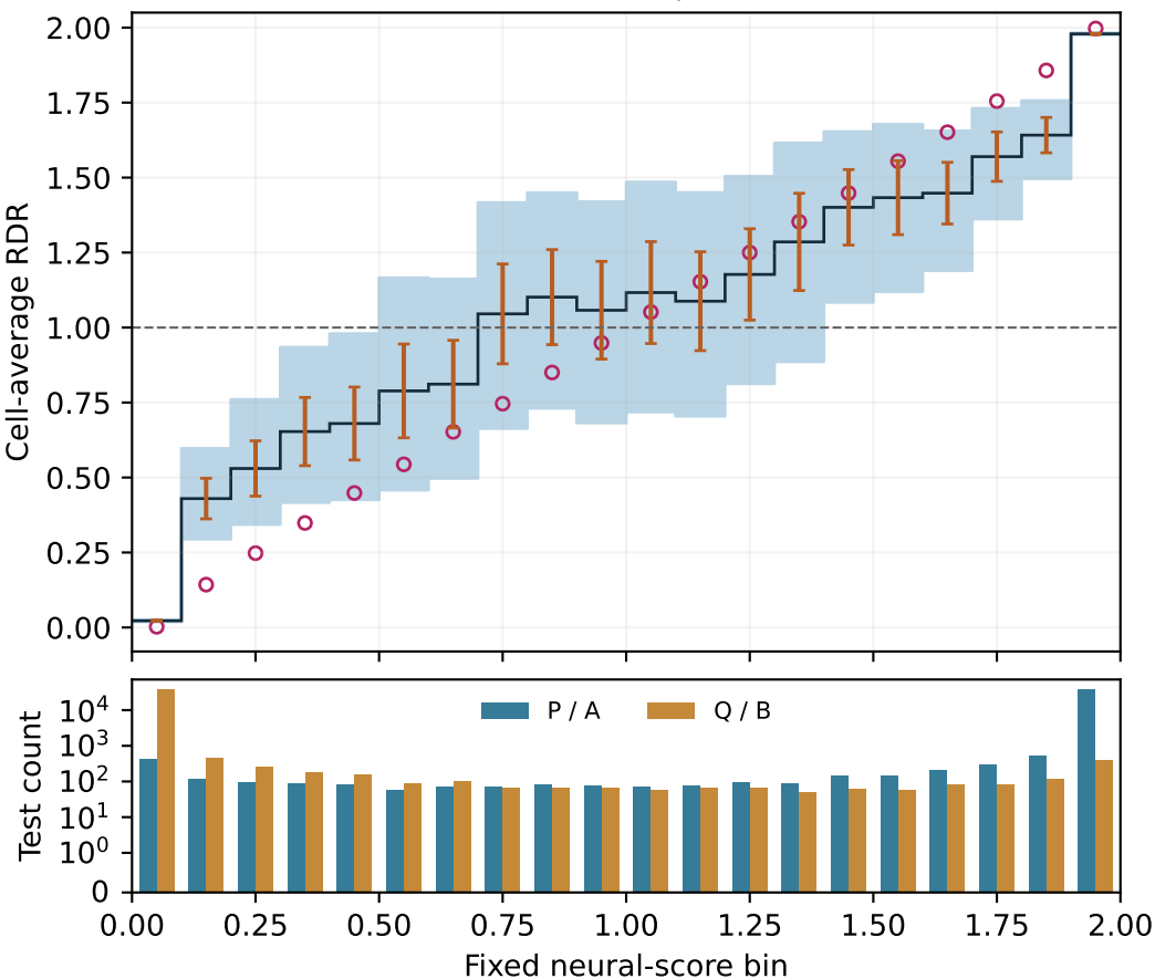
CelebA feature: merged held-out test, repeat 04 Nominal 95% cell-average intervals; same test pool for both estimates
