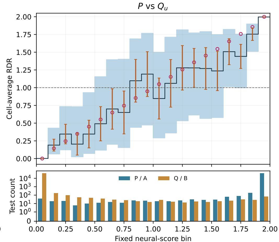
CelebA pixel: merged held-out test, repeat 02 Nominal 95% cell-average intervals; same test pool for both estimates
