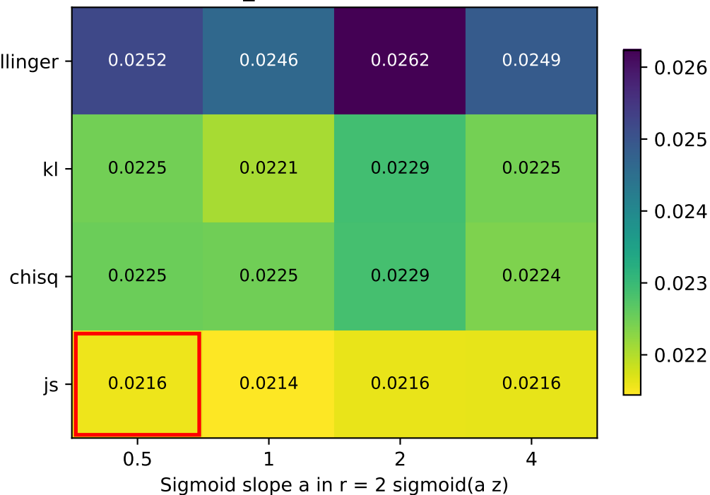
P vs Q_upper: Balanced Brier
