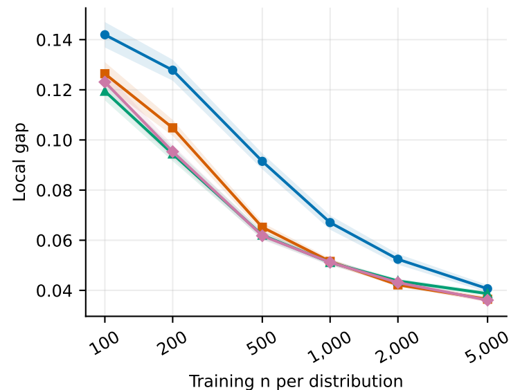
D=20, noise SD=0.10
