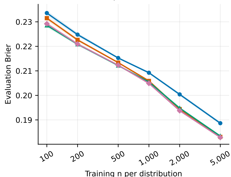
D=100, noise SD=0.30
