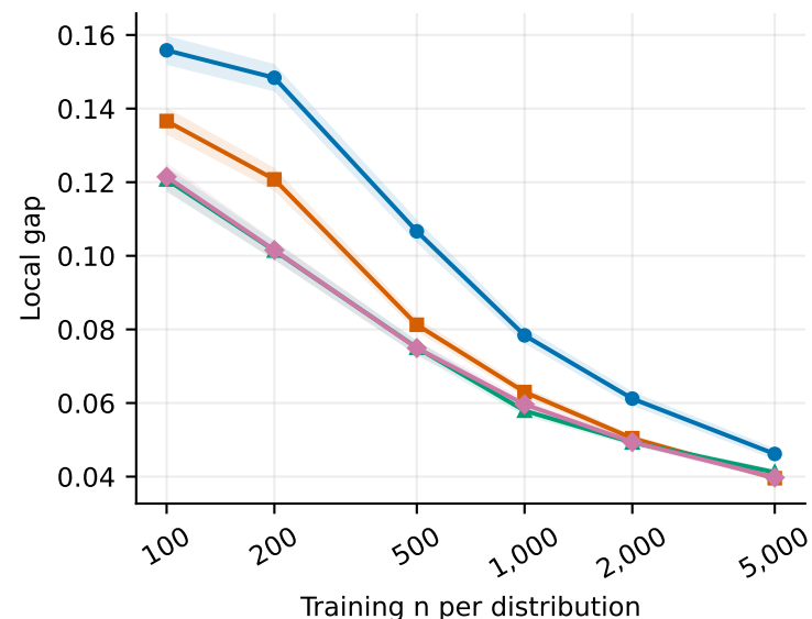
D=40, noise SD=0.30
