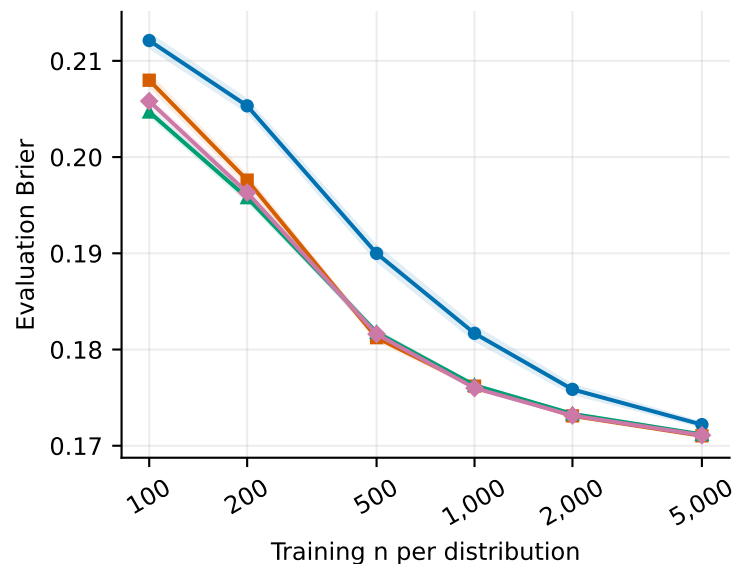
D=40, noise SD=0.10
