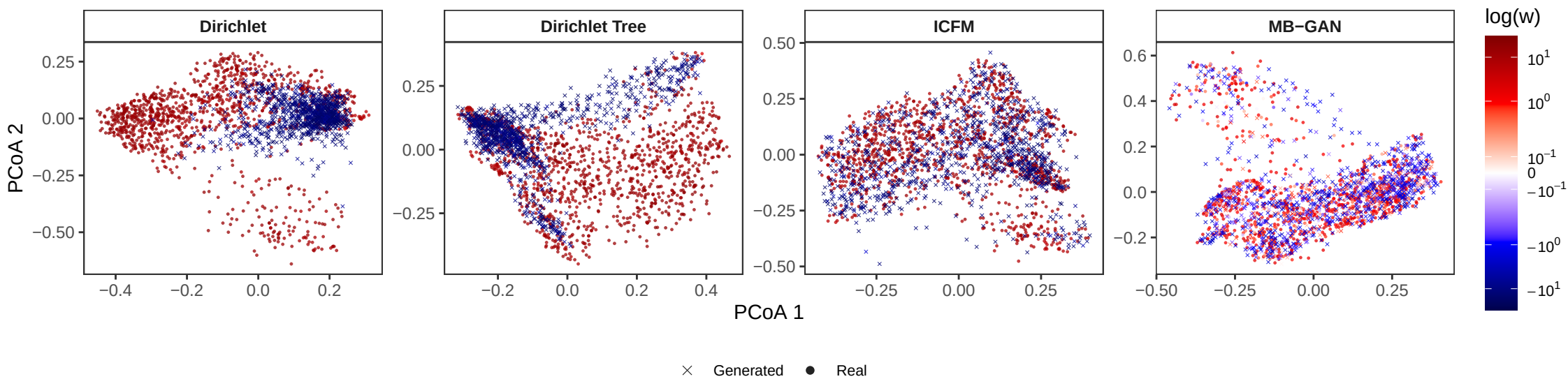
Train vs. Generated: Posterior mean of DRE
