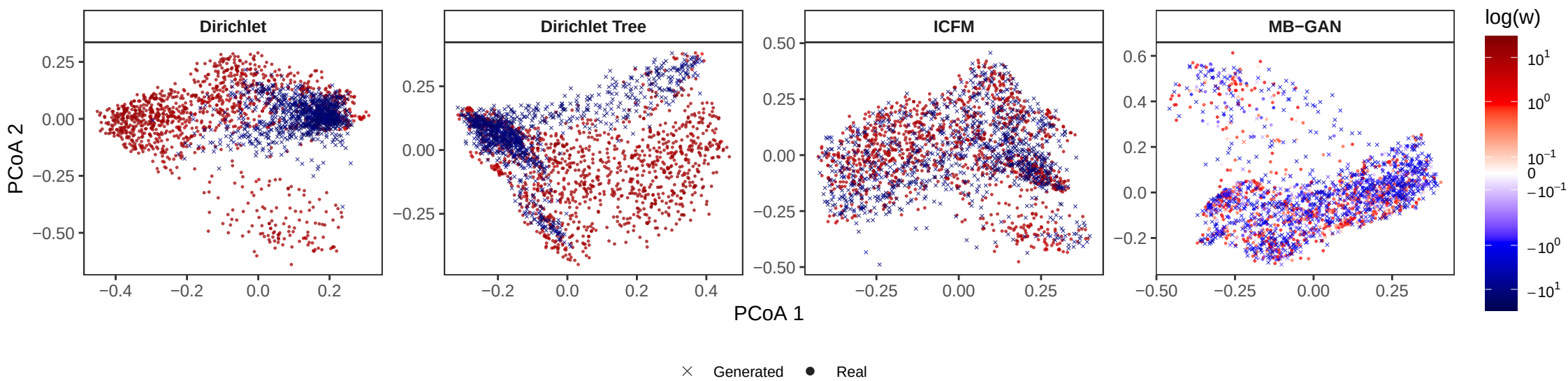
Train vs. Generated: Lower 2.5% MCMC quantile of DRE
