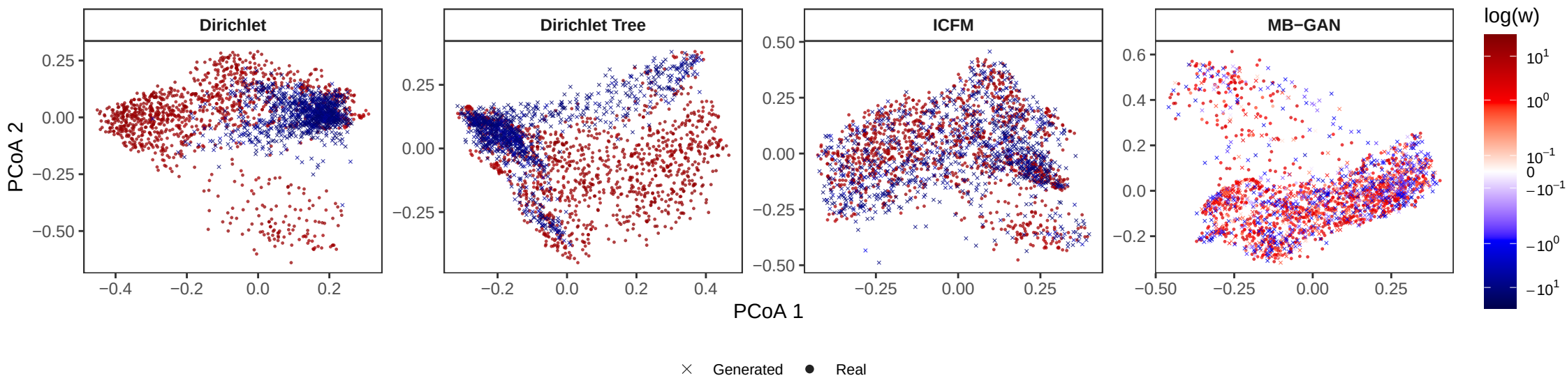
Train vs. Generated: Upper 97.5% MCMC quantile of DRE
