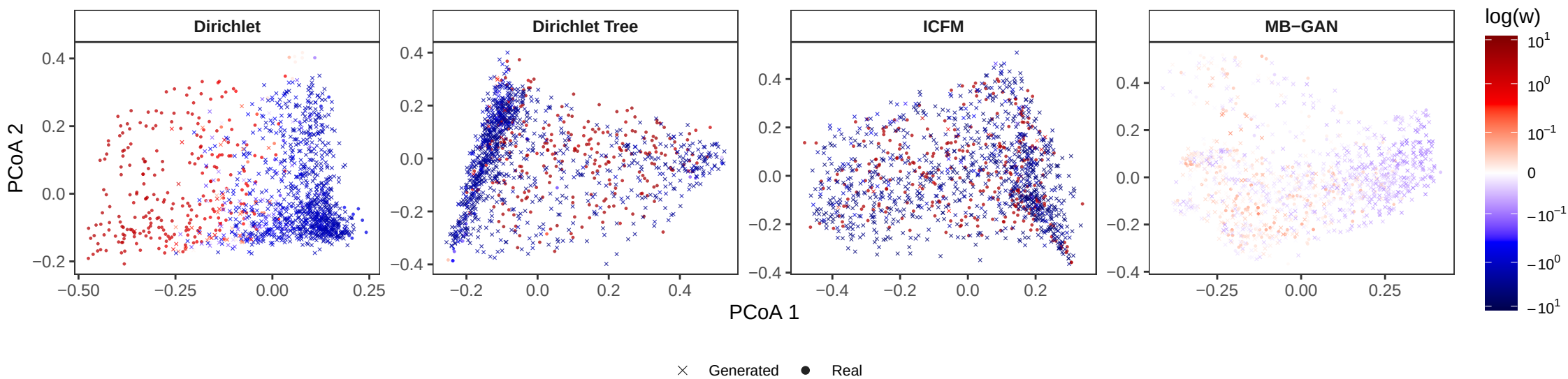
Test vs. Generated: Posterior mean of DRE
