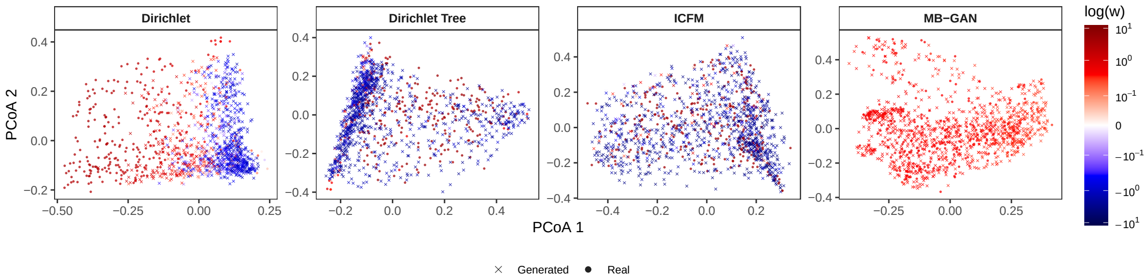
Test vs. Generated: Upper 97.5% MCMC quantile of DRE
