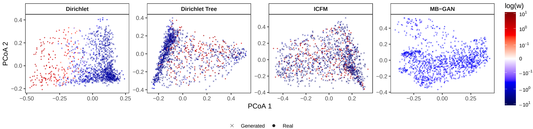
Test vs. Generated: Lower 2.5% MCMC quantile of DRE
