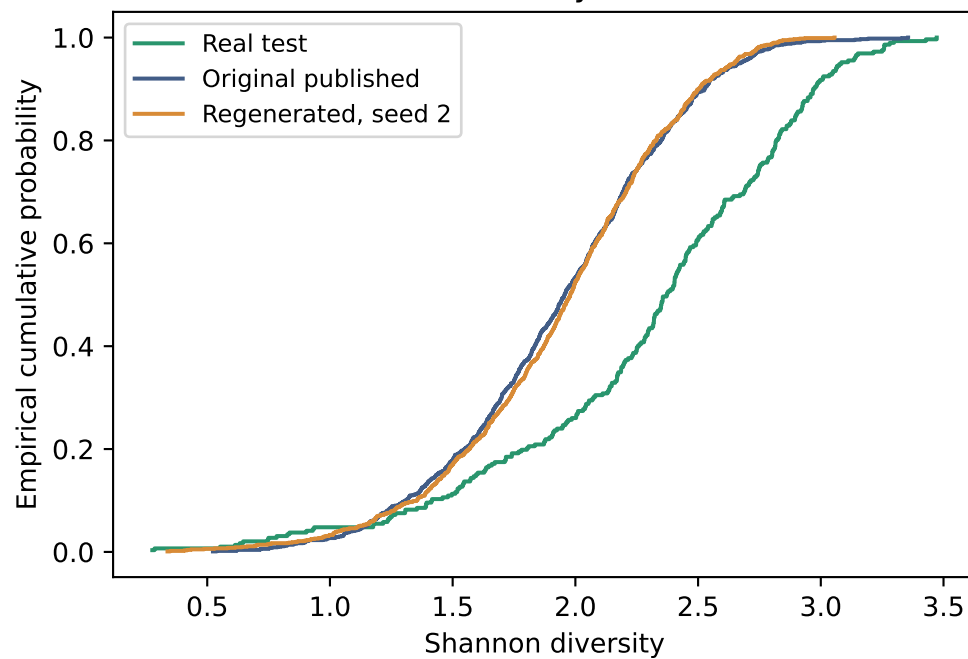
Shannon diversity distribution
