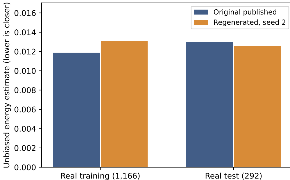
Joint discrepancy in square-root abundance space
