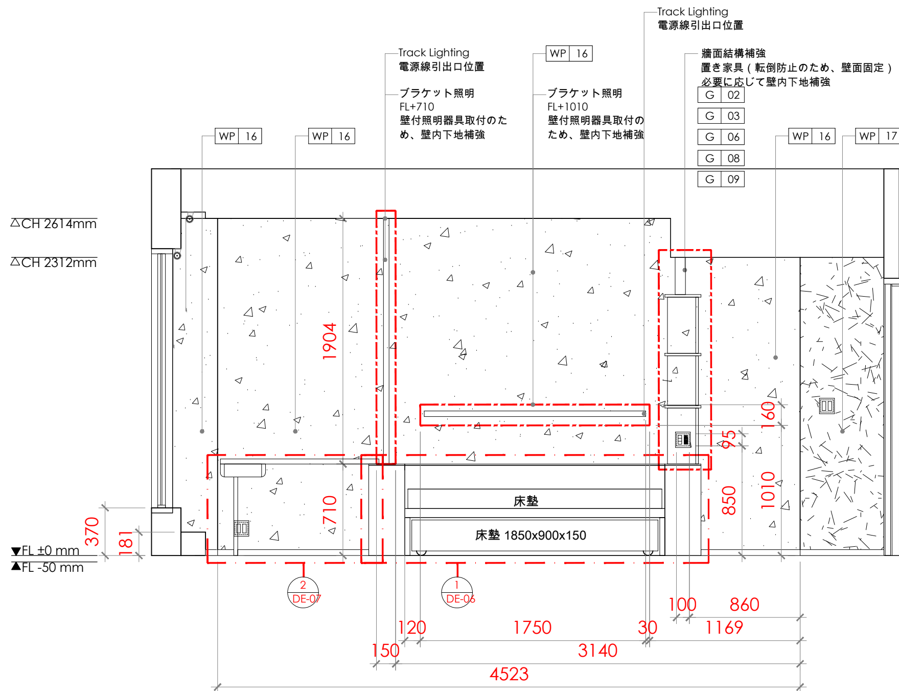
1 ELEVATION E-18 Scale=1:30
