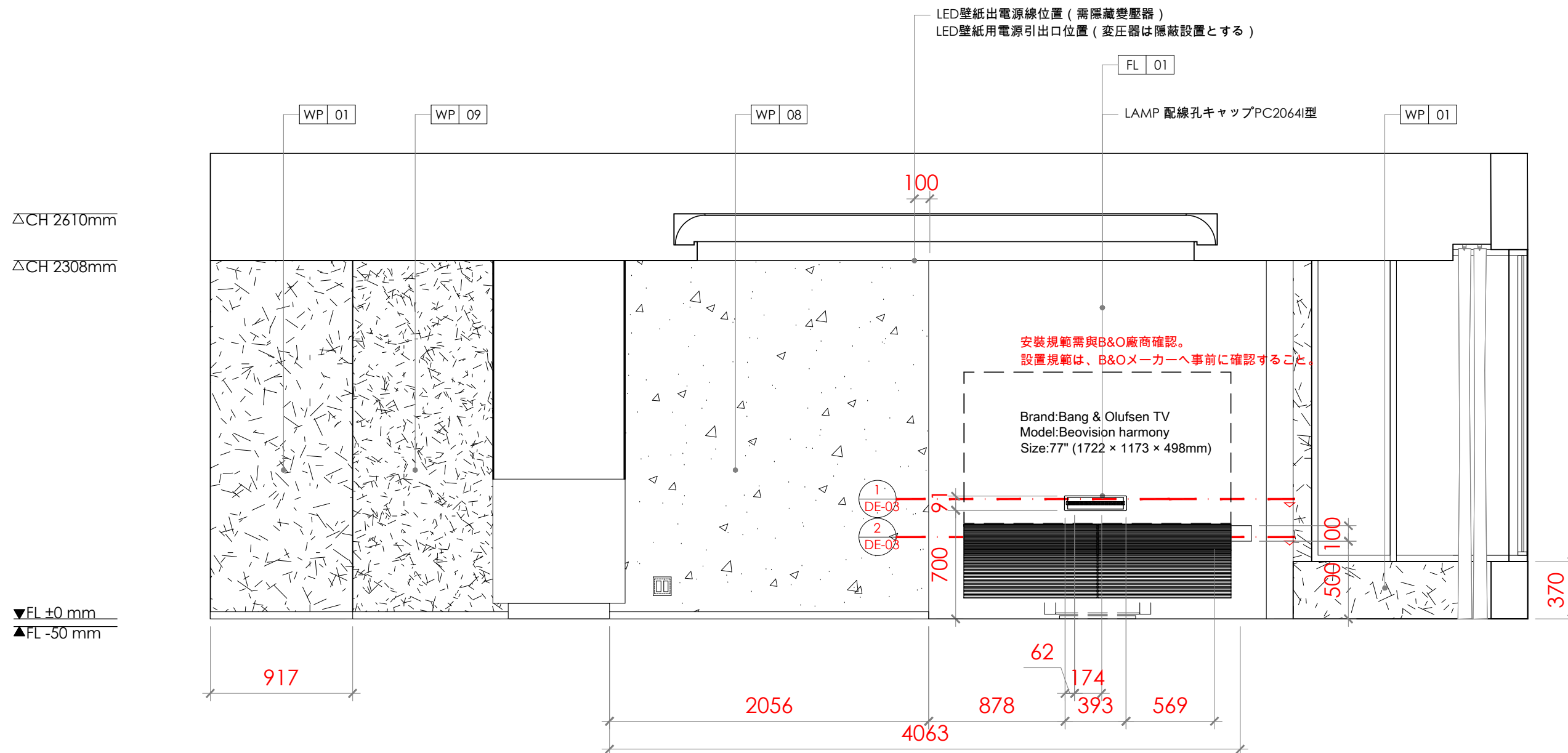
1 E-06 ELEVATION Scale=1:30
