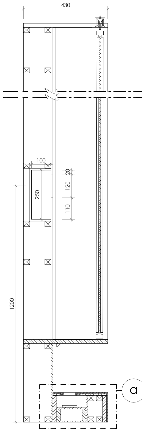
2 D-01 DETAIL S 1:10
