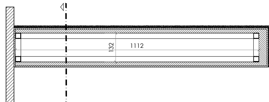
1 DETAIL S 1:10 D-01
