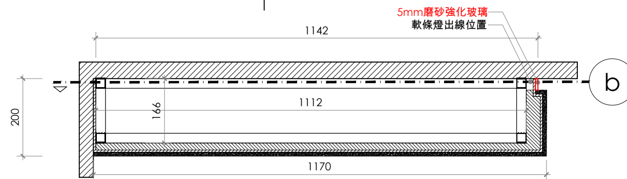
1 DETAIL S 1:10 D-01
