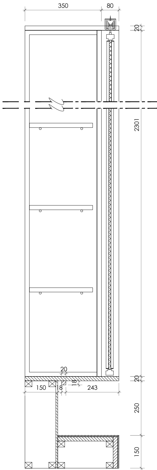
1 D-01 DETAIL S 1:10
