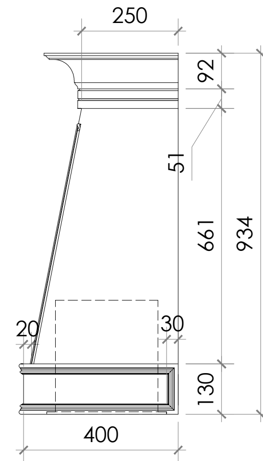
DETAIL S 1:10
