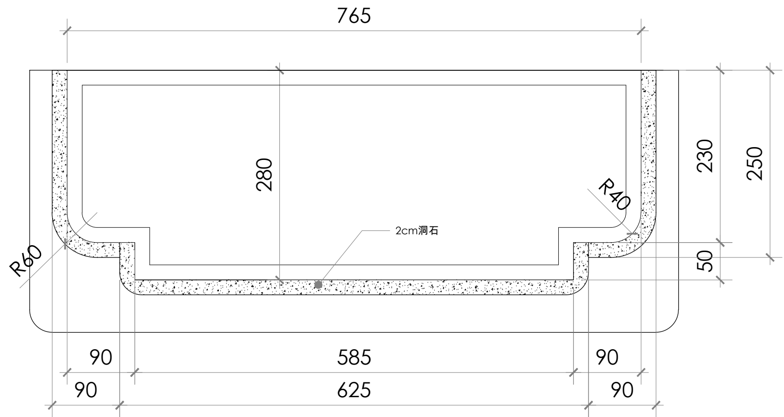
b DETAIL S 1:5
