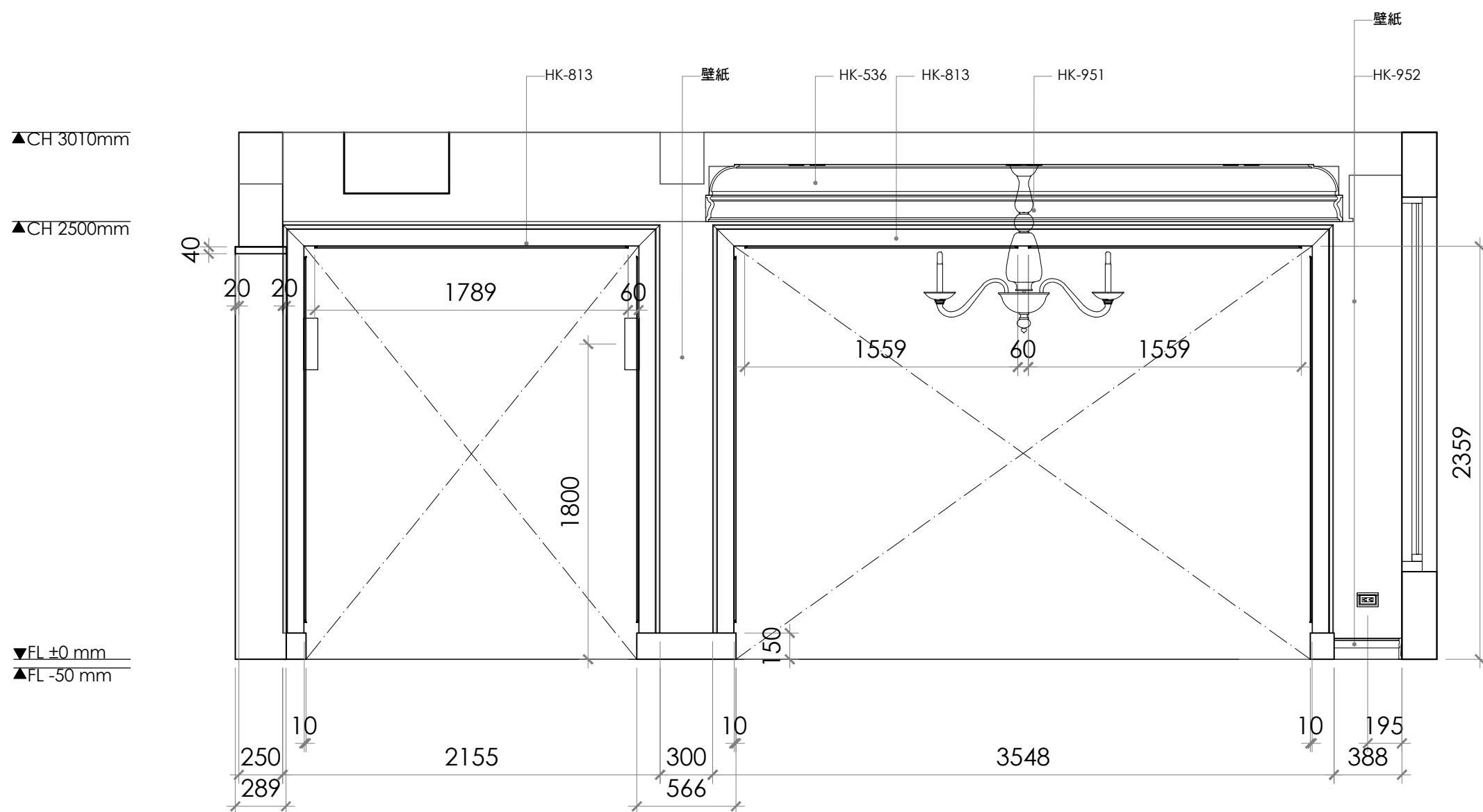
1 E-10 ELEVATION Scale=1:30
