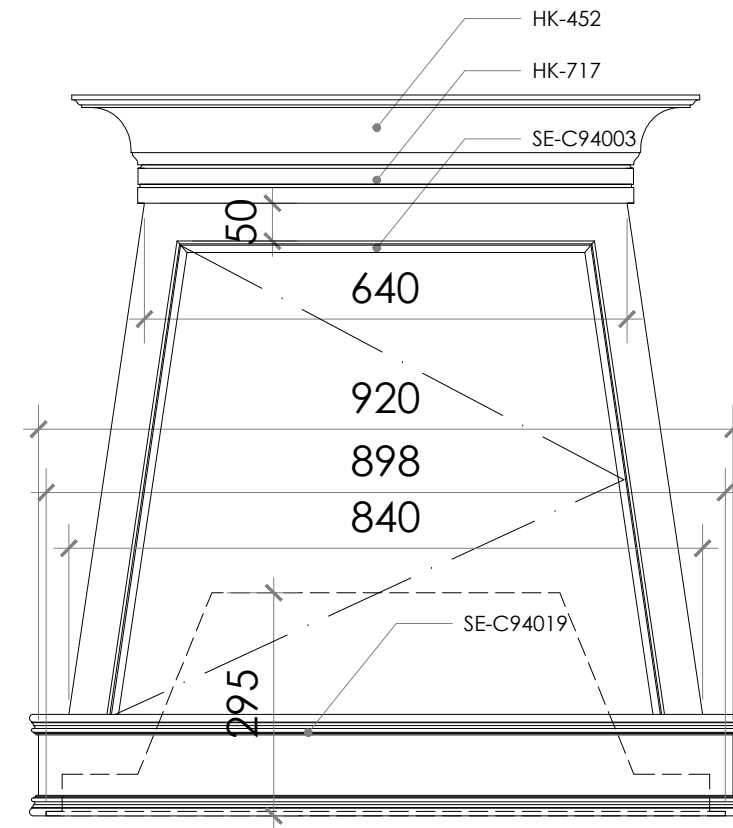
DETAIL S 1:10
