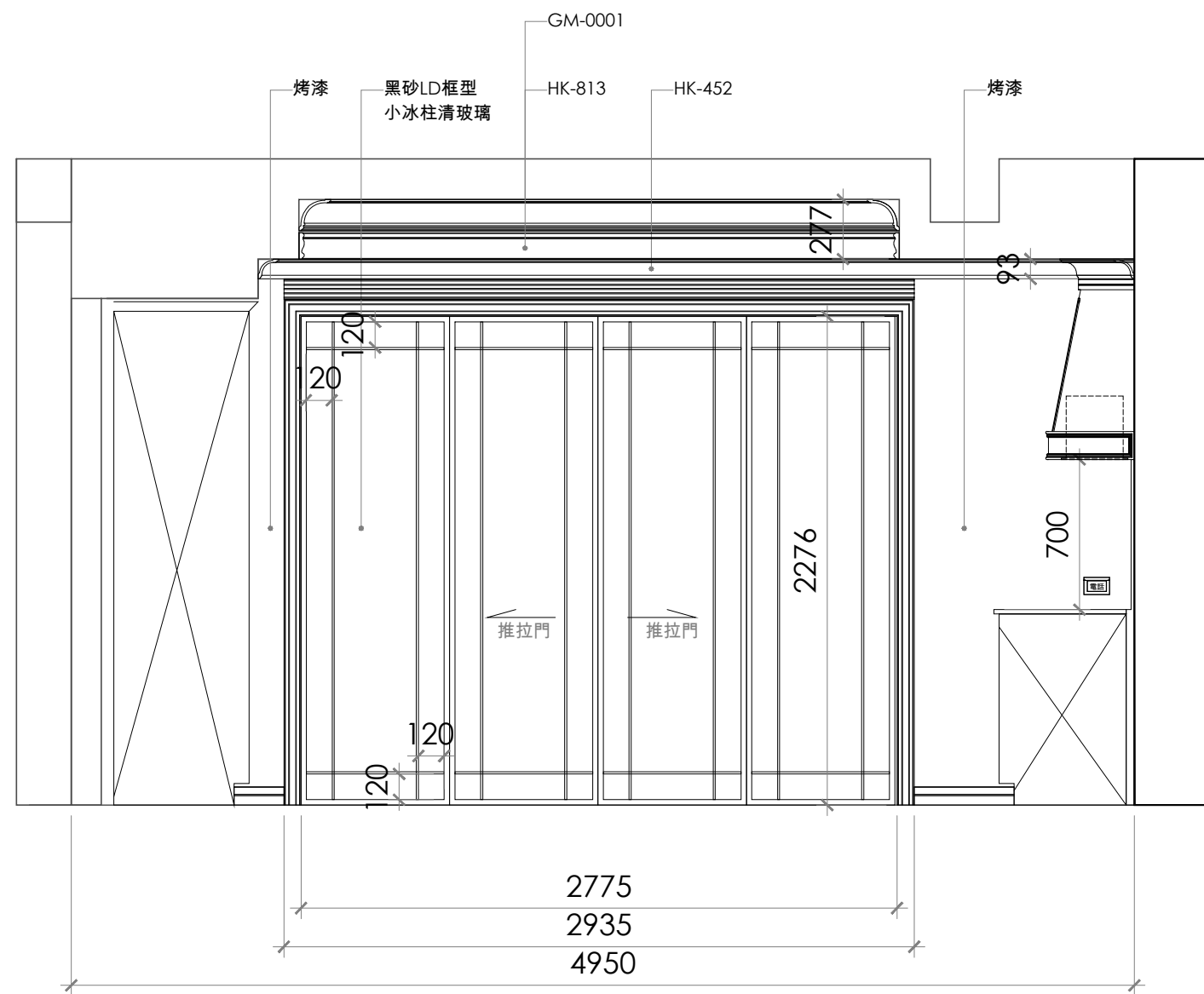
1 E-21 ELEVATION Scale=1:30
