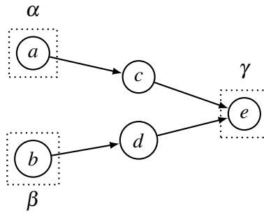
Fig. 14. Agent defense
