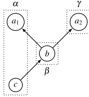
Fig. 4. Agent defense
