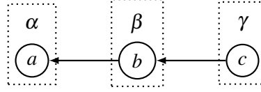
Fig. 2. Agent reinstatement
