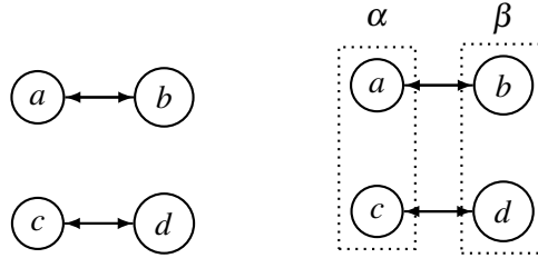
Fig. 1. An agent framework (AF) and an agent argument framework (AAF)
