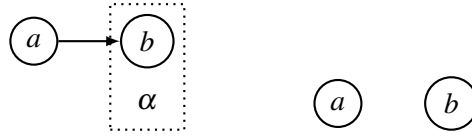
Fig. 22. An AAF (on the left) and SR_1(AAF) (on the right).
