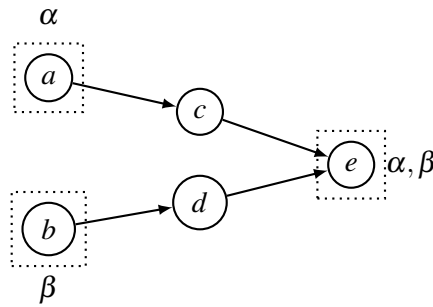
Fig. 17. Agent defense
