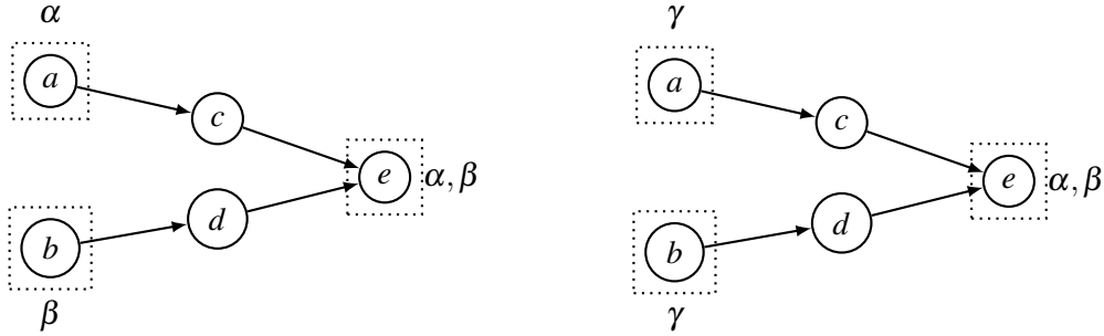
Fig. 18. Two AAFs: AAF_1 (on the left) and AAF_2 (on the right)
