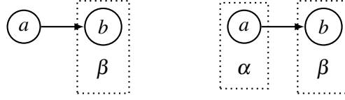
Fig. 7. Unknown argument and unknown attack
