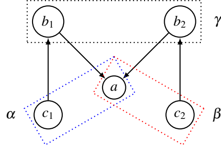
Fig. 3. c_1 and c_2 collectively defend a , but neither can agent-individually defend it.
