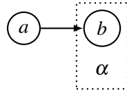
Fig. 8. An AAF = \langle \mathcal{A}, \rightarrow, \mathcal{S}, \sqsubset \rangle .
