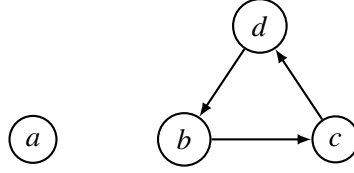
Fig. 10. Stable semantics for SR_1 and SR_3 do not satisfy Principle 3.
