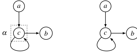
Fig. 12. SR_1 does not satisfy Principle 5.
