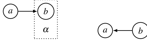
Fig. 21. An AAF (on the left) and SR_2(AAF) (on the right).
