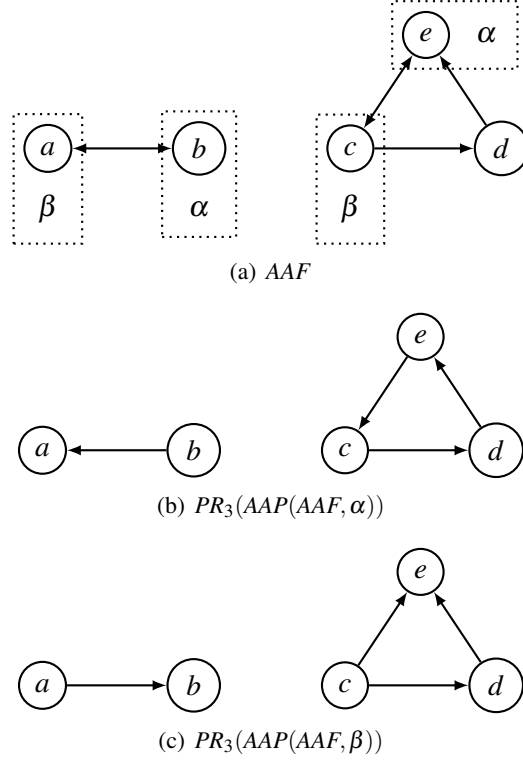
Fig. 25. A counterexample for Proposition 76.
