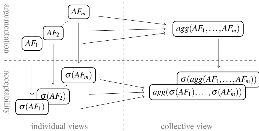
Fig. 6. A schematic overview of different approaches to collective acceptability in formal argumentation, where \sigma is a general placeholder for some kind of acceptability criterion on AFs, and agg is a general placeholder for some aggregation operator on AFs [13].
