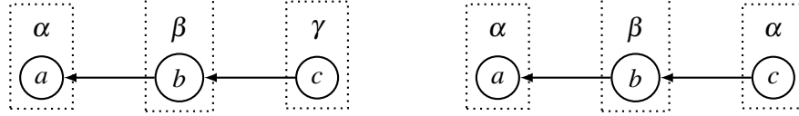
Fig. 19. \text{Sem}_1 does not satisfy Principle 15.
