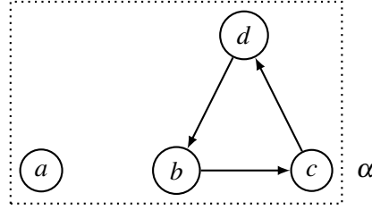
Fig. 26. Stable semantics for OR do not satisfy Principle 3
