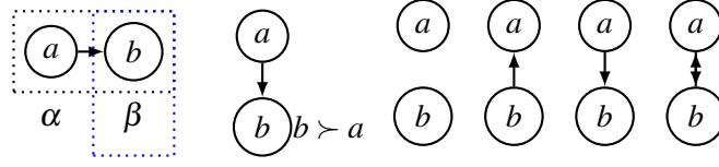
Fig. 5. Social reduction
