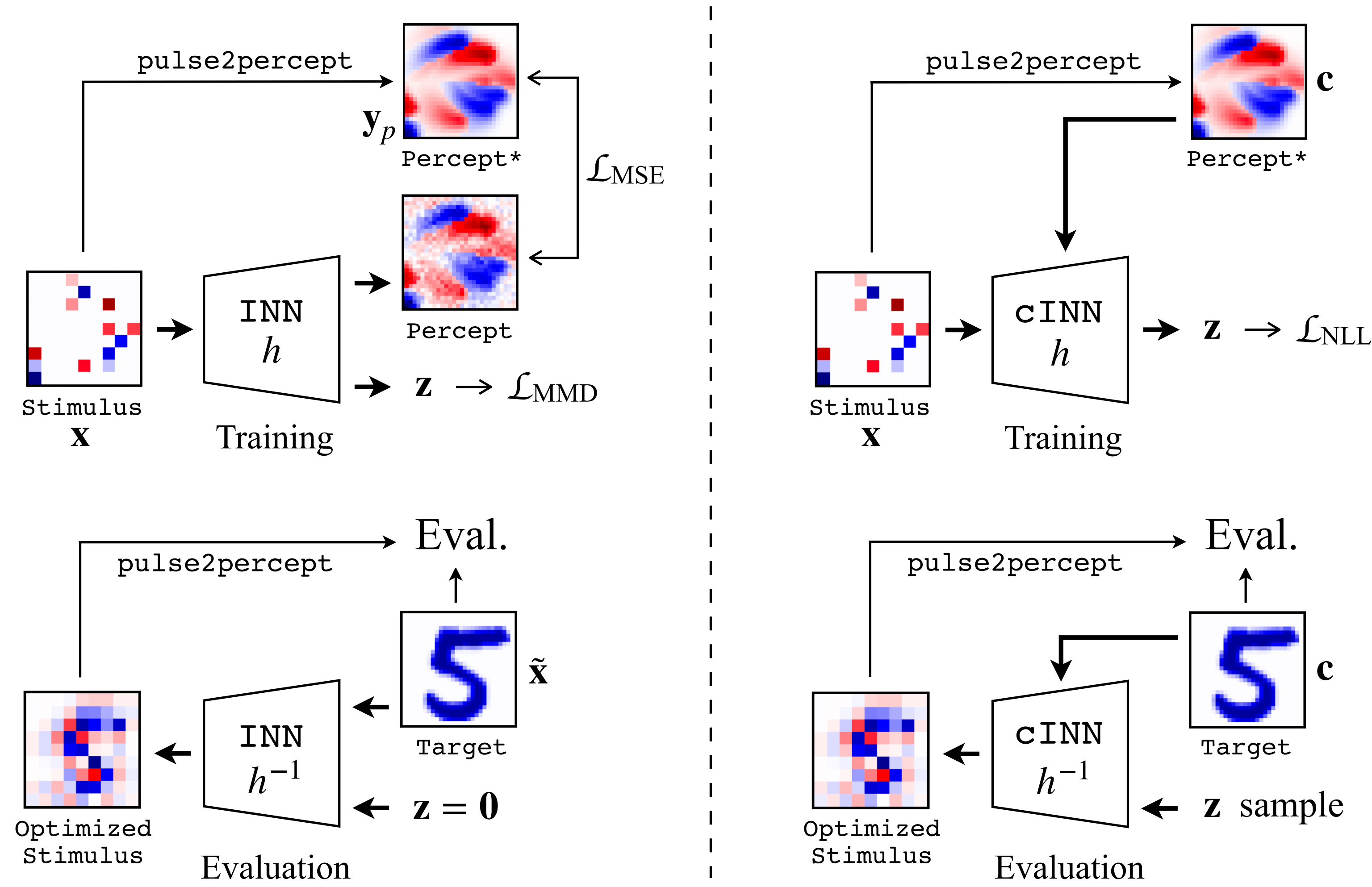
(a) MMD INN
