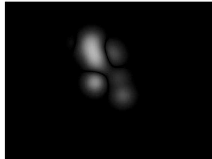
Saliency Map
