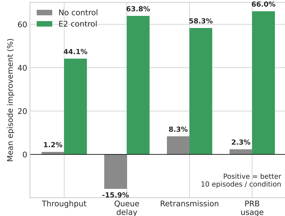
C. QoS proxy improvement
