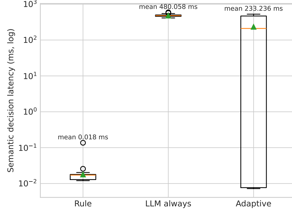
B. Decision-time distribution
