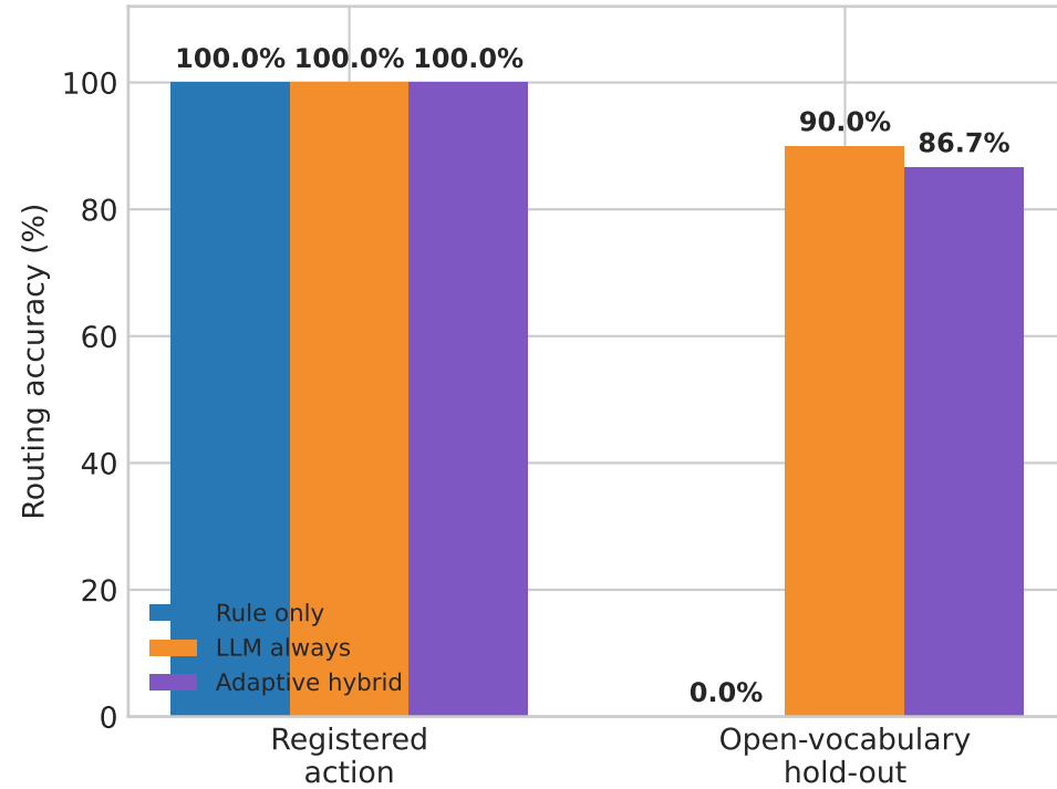
A. Accuracy by policy family
