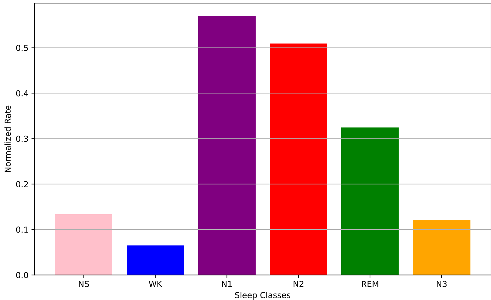
Normalized False Positive Rate by Sleep Class
