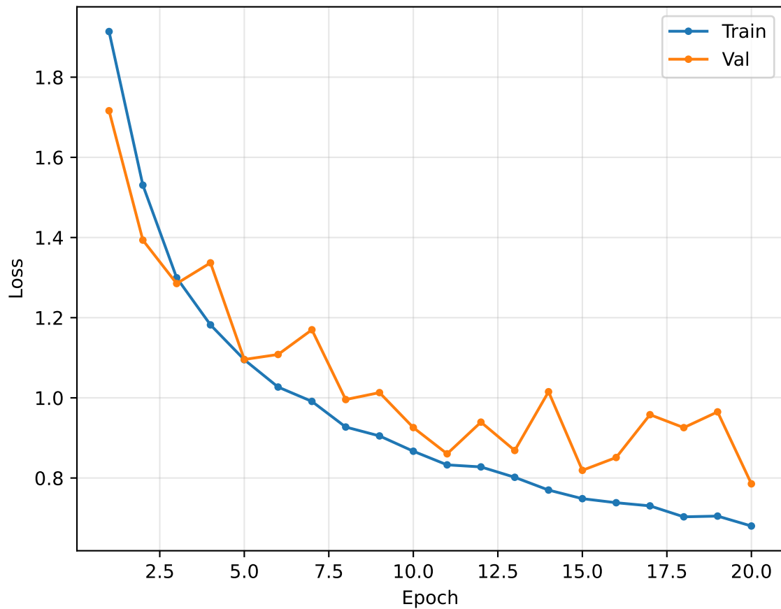
Model B Loss (Adam, lr=0.001)
