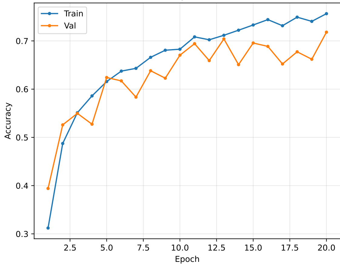
Model B Accuracy (Adam, lr=0.001)
