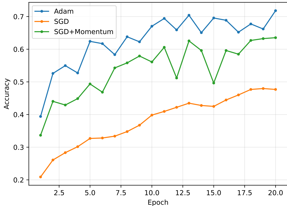
Validation Accuracy
