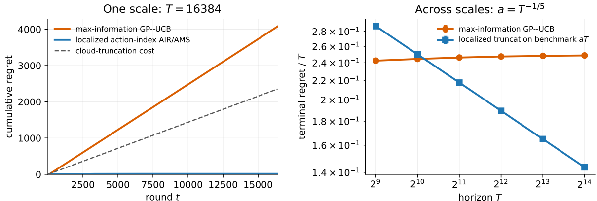
Figure 1: Finite-scale hub-cloud experiment. Monte Carlo curves show means and two standard errors over 200 independent runs; the truncation curves are deterministic. Left: cumulative pseudoregret at T = 16384 under the positive hub truth; the displayed AIR/AMS curve is evaluated under the positive retained hub truth, and the dashed line is the counterfactual one-hot-cloud truncation cost. Right: GP-UCB regret at the hub truth and the deterministic aT truncation benchmark, divided by T . Across scales, the finite kernel, a = T^{-1/5} , and the horizon-tuned AIR coefficient change with T .
