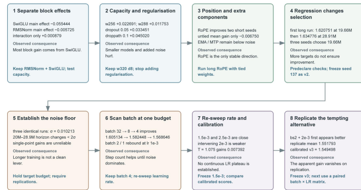
Fig. 6. The debugging path from v1/v2 structure, capacity, position and checkpoint selection to the v3 noise, batch, learning-rate and calibration checks; each observation directly determines the next experiment.
