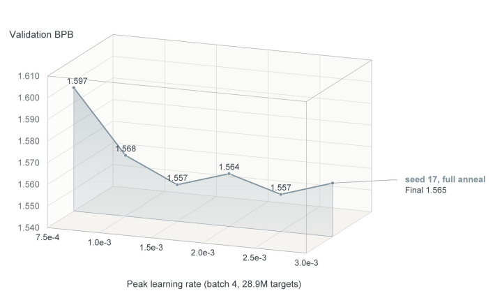
Fig. 3. Re-sweeping the peak learning rate after the batch was changed to 4; six points span 7.5\text{e-}4 to 3\text{e-}3 . The single runs at 1.5\text{e-}3 and 2.5\text{e-}3 differ by 0.000259, while the intervening 2\text{e-}3 point and the 3\text{e-}3 point are about 0.0075 worse and lowering the rate is clearly harmful.
