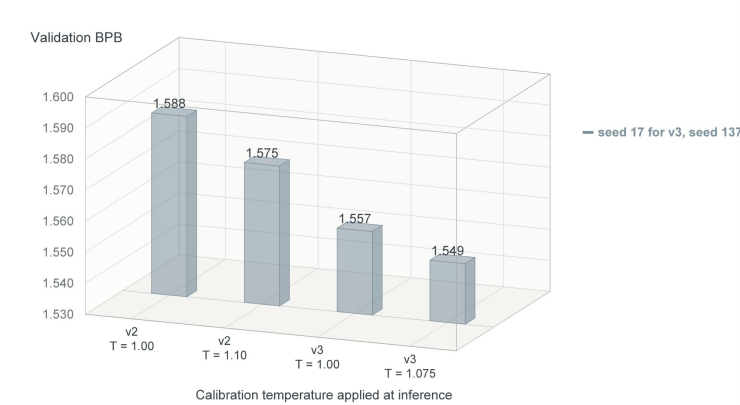
Fig. 4. Validation BPB before and after temperature scaling. The v2 value T = 1.10 is a post-freeze diagnostic and official v2 remains at T = 1.00 ; v3 selected T = 1.075 before its freeze.
