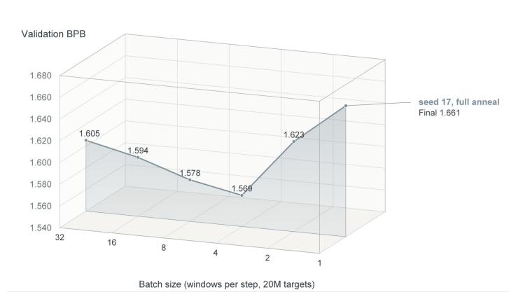
Fig. 2. Validation BPB against batch size. The curve bottoms out at four windows and degrades on both sides: smaller batches carry noisier gradients and going too far hurts the final quality.
