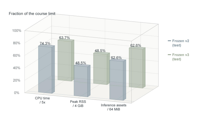
Fig. 5. Resource use of v2 and v3 on the test split, as a fraction of each limit. Both predictors remain below all three bounds, with nearly identical asset use.
