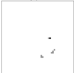
01 enemy presence
