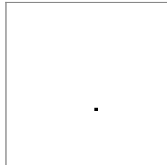
10 self marker
