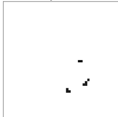
04 enemy threat
