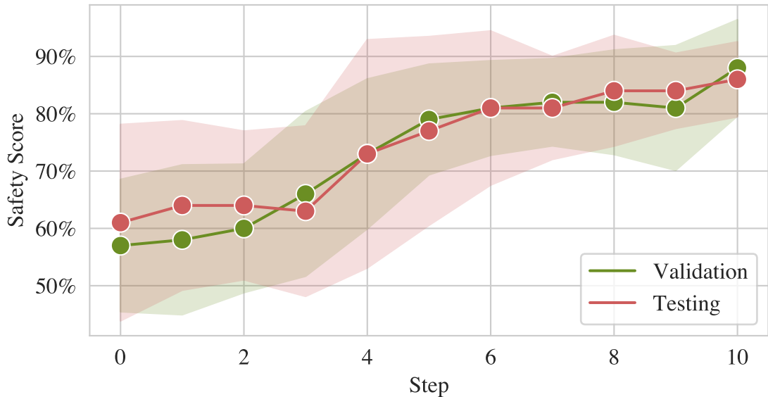
Our Safety Score vs. Number of Steps
