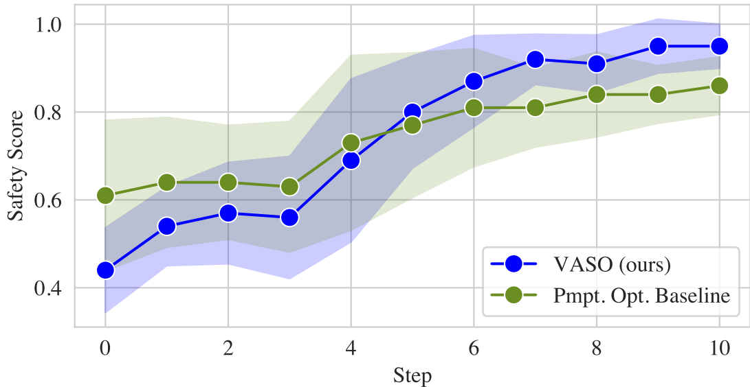
Safety Scores vs. Number of Training Steps
