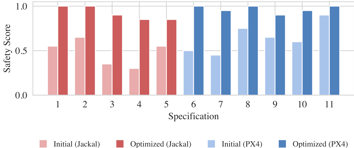
Safety Scores after 7 Training Steps over 100 Samples
