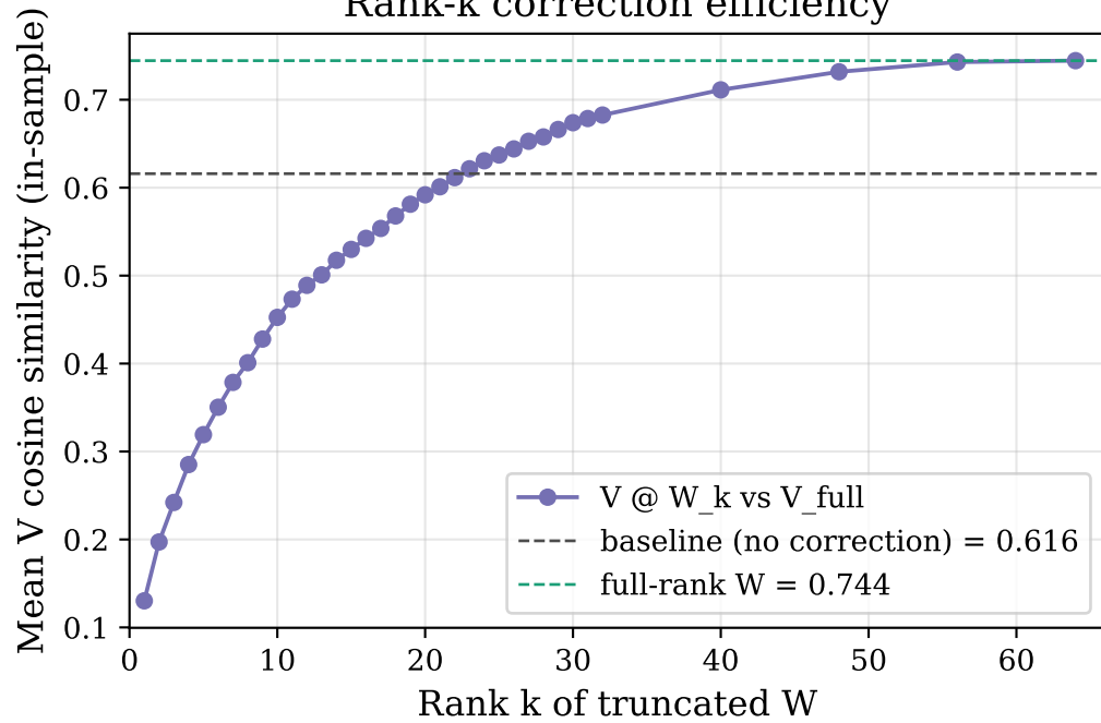
Rank-k correction efficiency
