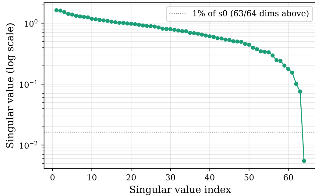
Singular value spectrum of learned W (L12)
