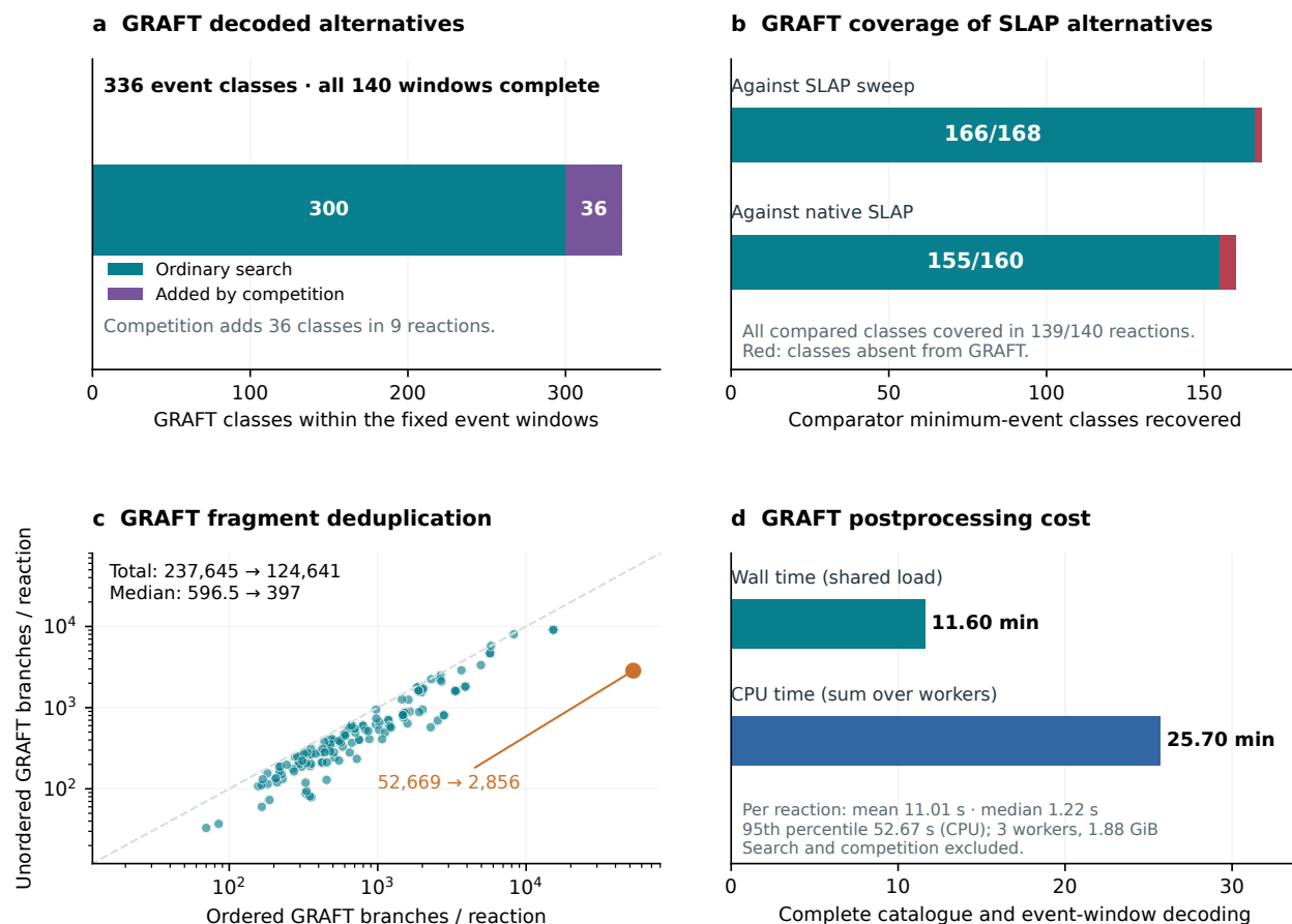
Figure 3 GRAFT outputs and decoding cost on 140 coordinate reactions. The default one-seed sweep is used with fragment competition. (a) GRAFT returns 336 distinct reaction-specific event classes within the fixed windows; competition adds 36 in 9 reactions. (b) GRAFT recovery of minimum-event classes among returned SLAP witnesses. All compared classes are covered in 139/140 reactions; the remaining reaction lacks two sweep alternatives at the same four-event minimum. (c) GRAFT ordered and unordered fragment-pair branch counts; the diagonal denotes equality. The highlighted case falls from 52,669 to 2,856. These are not counts of explicit mappings or event classes. (d) Complete GRAFT catalogue construction and window decoding on three workers: wall time, aggregate CPU time, and peak combined memory. Search and competition are excluded; wall time was measured under shared load.
