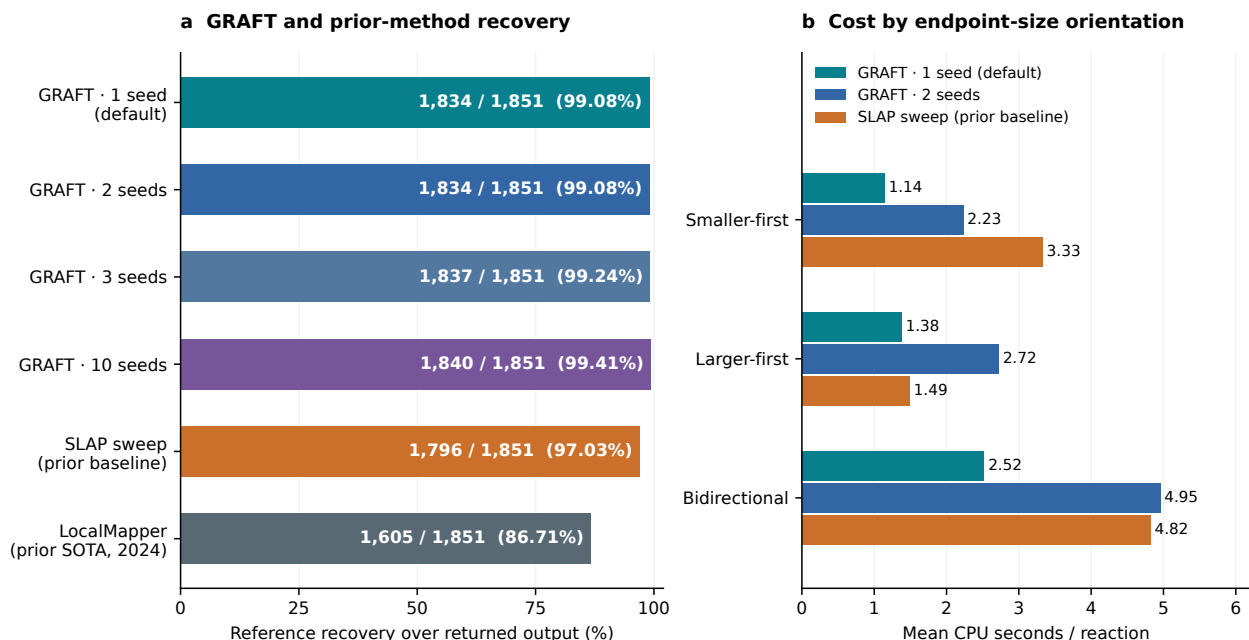
Figure 2 Reference recovery and search cost. (a) Golden recovery for swept GRAFT and SLAP, with LocalMapper as the prior accuracy-SOTA baseline (2024). LocalMapper returns one mapping; the other bars measure coverage among alternatives. All values use our evaluator, not literature-reported accuracies. Unswept controls are reported in Table 2. Every percentage uses all 1,851 records. (b) Mean CPU for smaller-first, larger-first, and bidirectional search on the same 1,821 completed reactions on the Mac. Reference verification is excluded; the procedures have different search objectives, output cardinalities, and I/O timing scopes.
