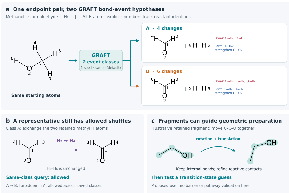
Figure 4 Information retained beyond one atom mapping. (a) Current GRAFT output for methanol \rightarrow formaldehyde + H_2 : two event classes at \tau_{iso} = 1 , event threshold 0.5, one seed and a 2,000-branch cap with cut sweep. Atom numbers track reactant identities; all six atoms are shown. The classes differ in hydrogen origin as well as event count. Red text lists lost bonds and blue text lists formed or strengthened bonds; C-O \rightarrow C=O contributes one positive event. (b) A joint H_3/H_4 exchange is certified within class A; transferring to class B requires relaxing the event-class restriction. One witness alone reports neither fact. (c) Retained fragment membership can guide a downstream rigid translation/rotation before local reaction-coordinate refinement. This is a proposed use, not a transition-state calculation; permutations of atom identities and continuous fragment motions are different operations. Counts and query verdicts in (a,b) are checked by the public Python API.
