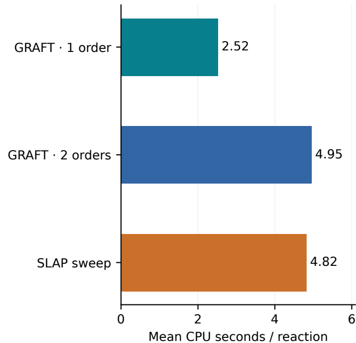
b Same-Mac workflow cost
