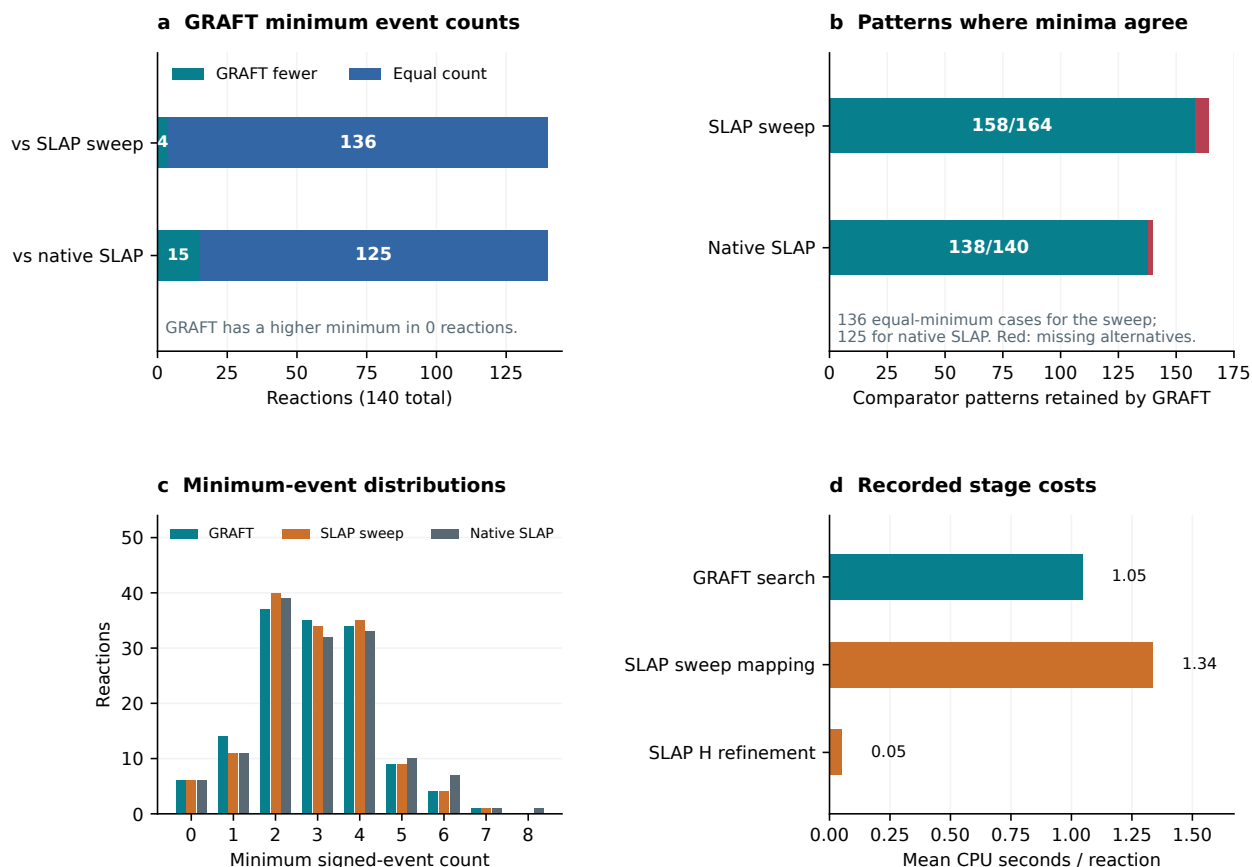
Figure 3 Bond-event counts, alternative patterns, and runtime on 140 coordinate reactions. GRAFT uses one seed and the sweep at cap 2,000. (a) Reactions where GRAFT finds fewer or equal events than each SLAP baseline; none has a higher GRAFT minimum. (b) Comparator minimum-event patterns recovered by GRAFT, counting only reactions where both methods reach the same minimum. The six missing SLAP-sweep patterns span four reactions. (c) Distribution of the minimum event count across reactions for each method. (d) Mean CPU seconds per reaction for the recorded stages. The timing panel reports search and SLAP refinement; it excludes GRAFT event decoding. See Table 6 for timing scope. The mappings are unverified, so this figure compares bond events rather than mapping accuracy.
