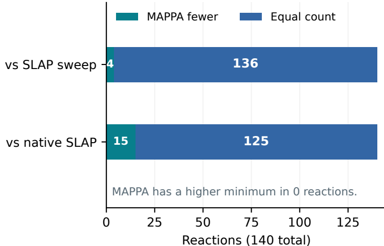
a MAPPA minimum event counts
