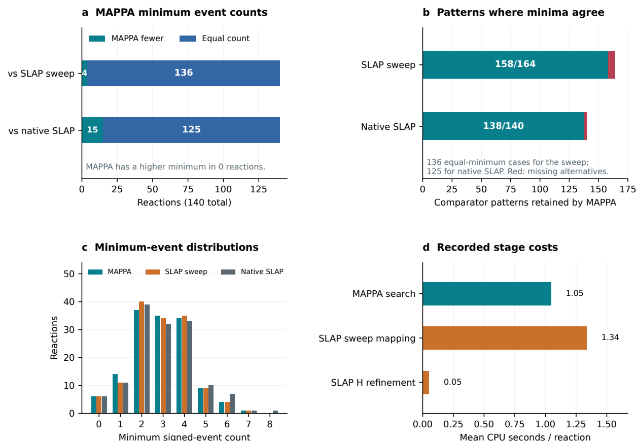
Figure 4 Bond-event comparison on 140 coordinate reactions. MAPPA uses one seed, the sweep, and cap 2,000. (a) Reactions with fewer or equal MAPPA events than each SLAP baseline. (b) Comparator minimum-event patterns recovered by MAPPA at equal minima. (c) Minimum-event count distributions. (d) Mean CPU for search and SLAP refinement, excluding MAPPA decoding (Table 5). Atom mappings are unverified; this compares bond events, not mapping accuracy.
