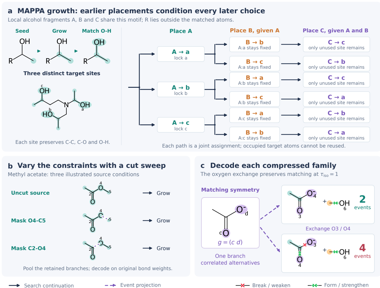
Figure 1 MAPPA: conditional fragment branching and compressed symmetry. (a) A local alcohol motif grows while retaining its O-H bond. Three sites in the depicted target have distinct molecular environments. For three source fragments sharing this motif, placing A fixes one site; B then branches over the two unused sites, and C takes the remaining site. The tree illustrates local conditioning and injectivity; R denotes atoms outside the matched subgraph, and this is not a complete reaction-search trajectory. All attached hydrogens in the illustrated local matches are checked. (b) The cut sweep searches the uncut source graph and graphs with one source edge masked. The illustrated ester masks change the growth and preservation constraints; their outputs are pooled. Masking an edge does not itself assign a bond event. (c) Exchanging the two acetate oxygen images preserves the fragment’s element and bond-weight matching tests at \tau_{iso} = 1 , but changes two heavy-atom events into four at threshold 0.5. Neither acetate oxygen carries H. Solid black lines retain the endpoint bonds. Red \times marks on the bonds indicate cleavage or weakening; paired green arrows pointing inward indicate formation or strengthening. Pastel colors track fragment membership or symmetry sites. Dashed arrows are event projections within a family, not additional search branches. Saved constraints govern allowed symmetry actions. These formal-bond-order event signatures illustrate MAPPA decoding, not distinct mechanisms or resonance-normalized transformations.
