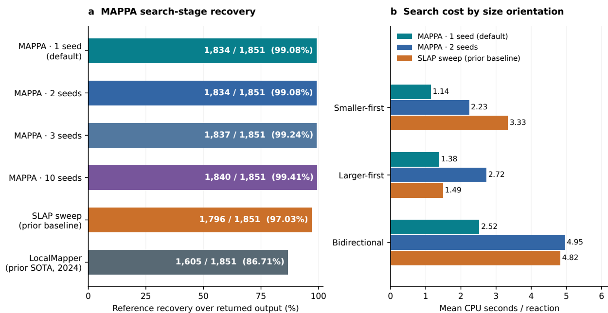
Figure 3 Golden reference recovery and search cost. (a) Reference recovery over all 1,851 reactions. MAPPA and SLAP use our cut sweep; LocalMapper is the prior accuracy-SOTA baseline and returns one bijection. All scores use our evaluator. (b) Mean search CPU over the same 1,821 completed reactions, by orientation. Bond-event decoding is excluded. Full comparisons and timing scopes are in Tables 2 and 3 .
