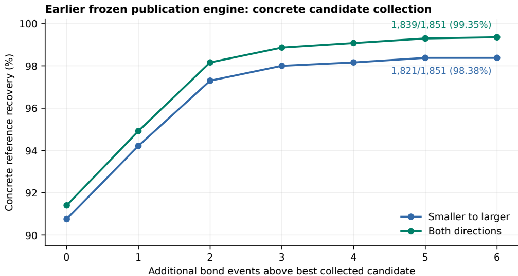
Figure S2 Recovery among collected concrete candidates. This uses the earlier publication engine, separately from the seed ablation. Event windows are relative to the best collected score at maximum coverage. All 1,851 records remain in the denominator. Extraction does not enumerate every represented mapping.
