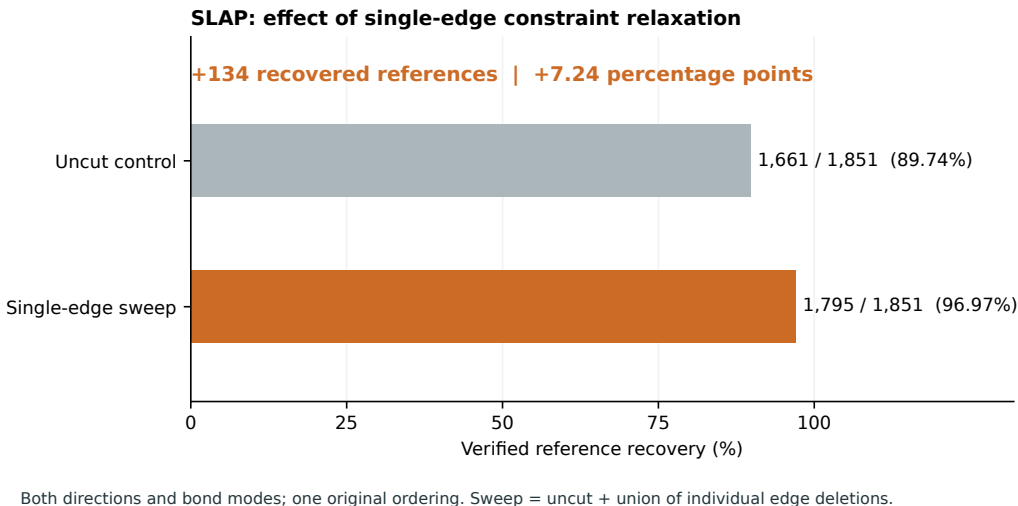
Figure S1 Supporting single-edge ablation in SLAP. The control and sweep use the same original ordering, both directions, and binary and weighted modes. The sweep unions the uncut output with outputs from individual source-edge deletions. Recovery increases by 134 cases (7.24 percentage points). All 1,851 records remain in the denominator, including incomplete variants. This experiment evaluates the cut policy in SLAP, not the individual components of GRAFT.
