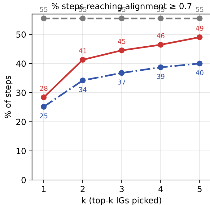
pass@k comparison on 155 elementary steps (verifier vs uniform-random baseline; oracle ceiling shown for reference)
