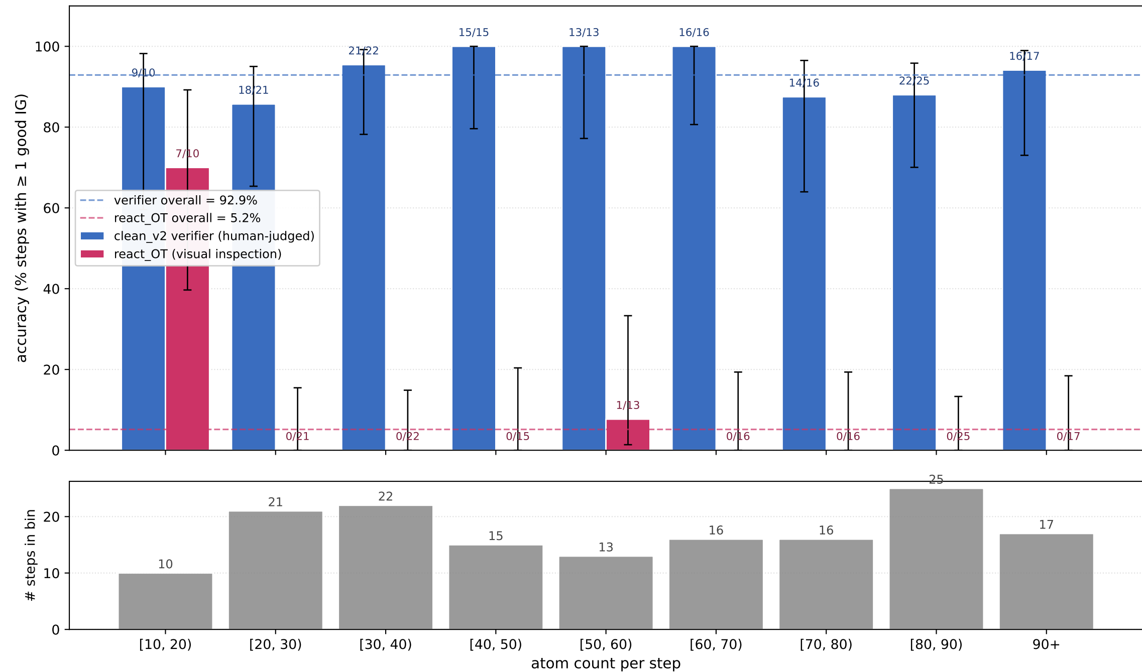
Accuracy by atom-count bin (N = 155 steps; binwidth = 10 atoms; last bin pools 90+; error bars = 95% Wilson CI)
