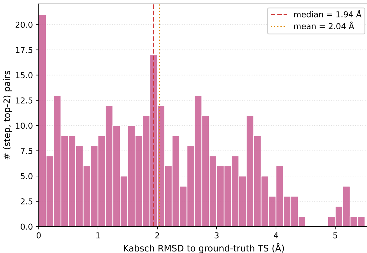
Ranker's top-2 IGs vs. GT (N = 310)
