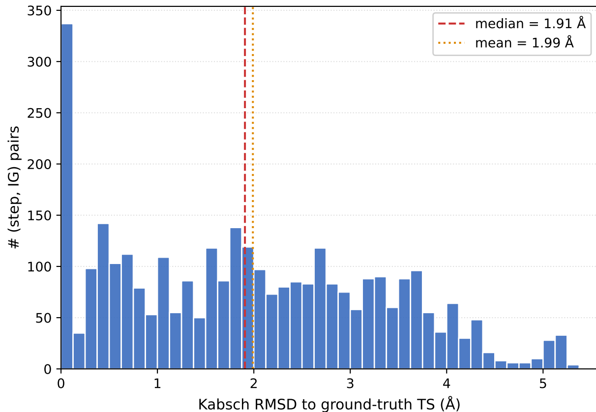
All 20 IGs vs. GT (N = 3251)
