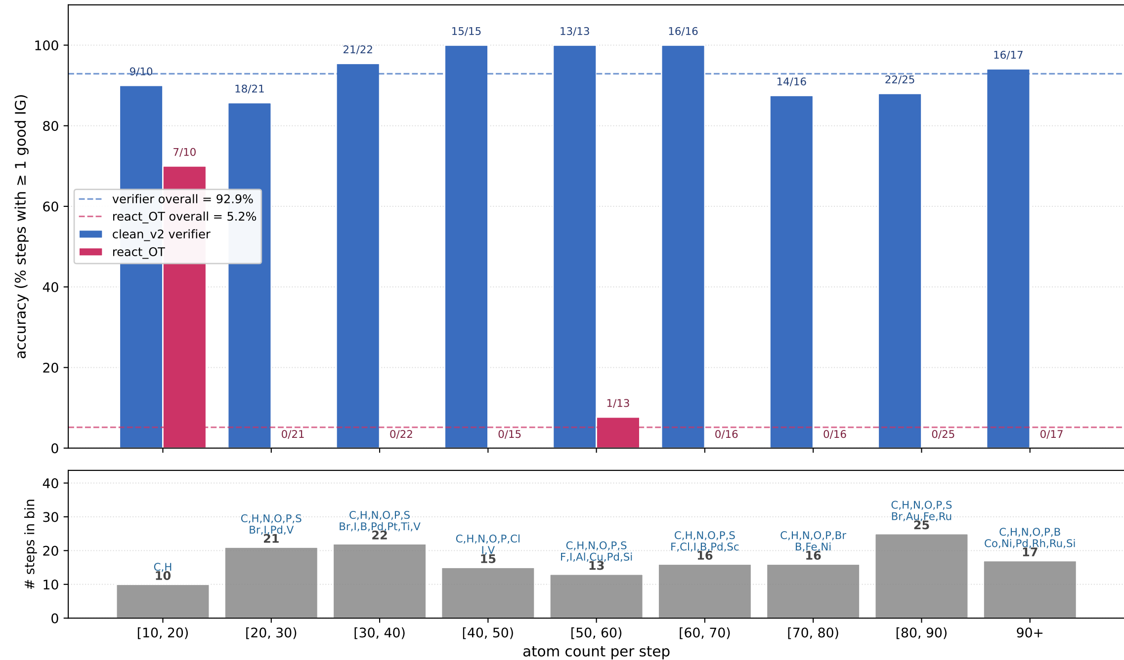
Accuracy by atom-count bin (N = 155 steps; binwidth = 10 atoms; last bin pools 90+)
