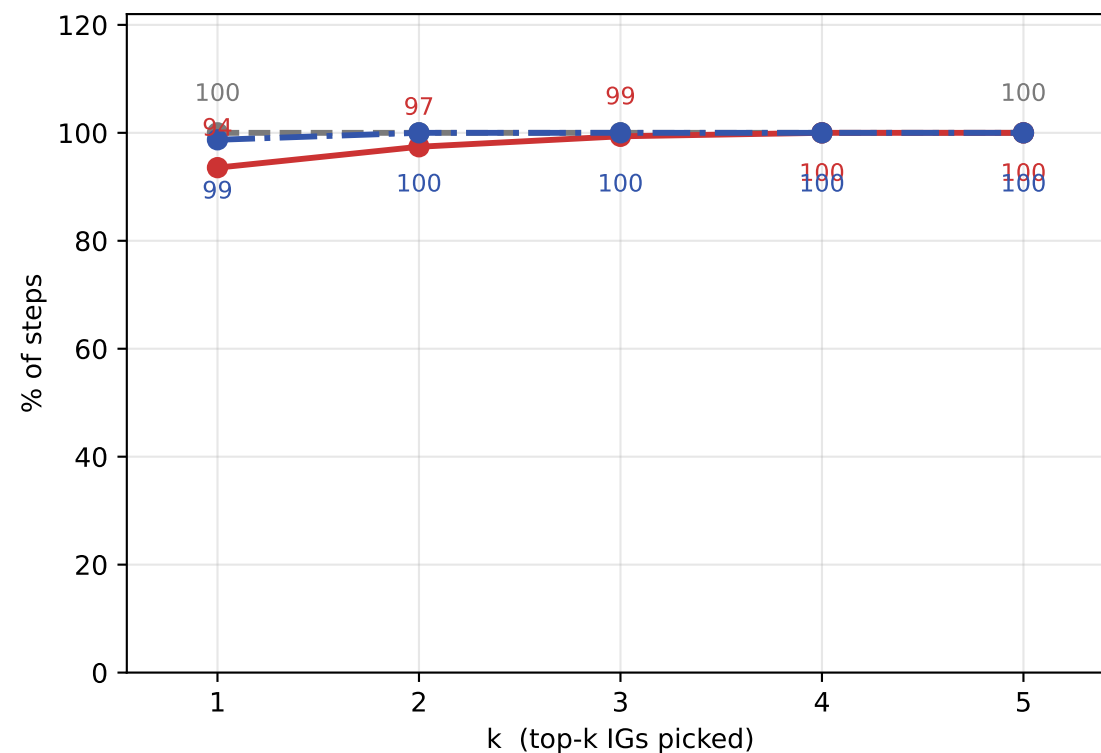
% steps reaching alignment \geq 0.3
