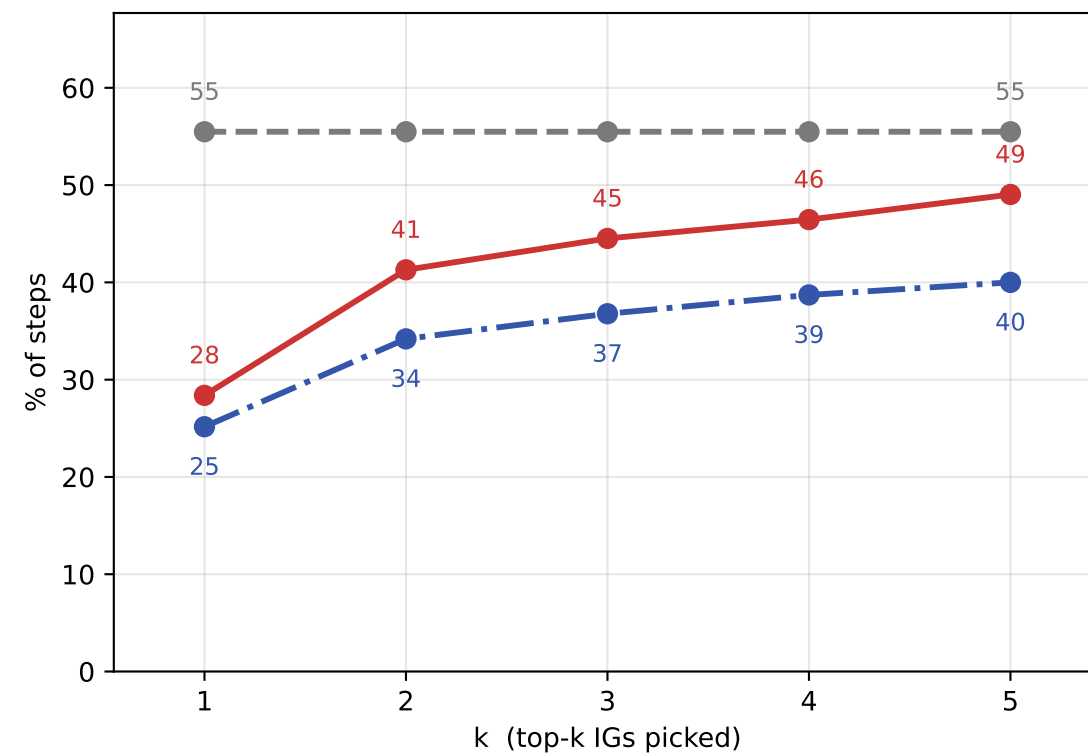
% steps reaching alignment \geq 0.7
