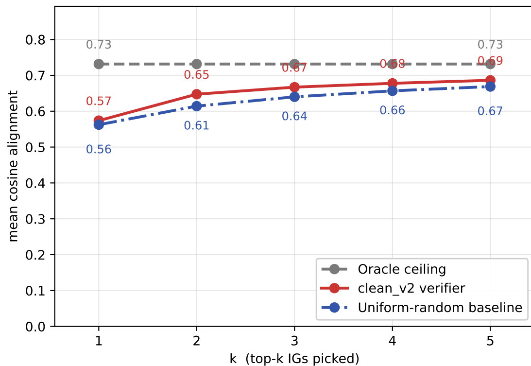
mean alignment
