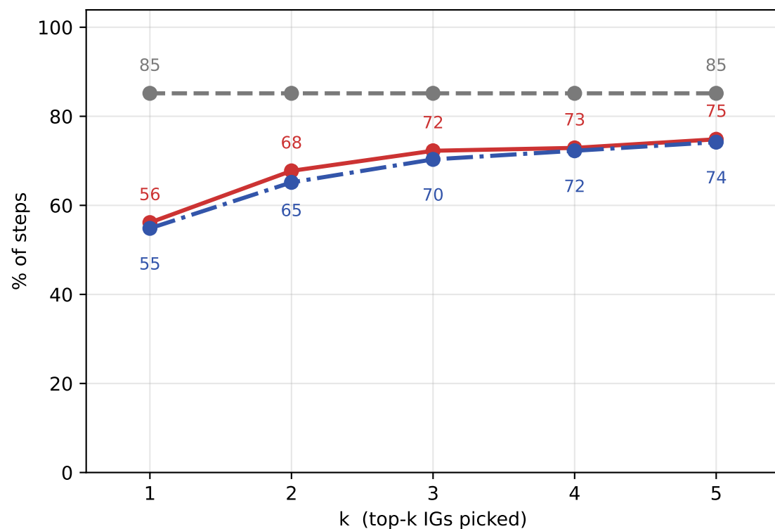
% steps reaching alignment \geq 0.5
