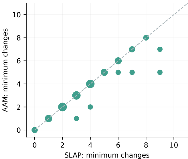
a Best saved mapping scores
