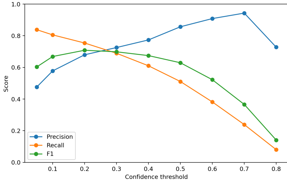
Figure 4: External-domain calibration curve used to select high-precision operating points.
