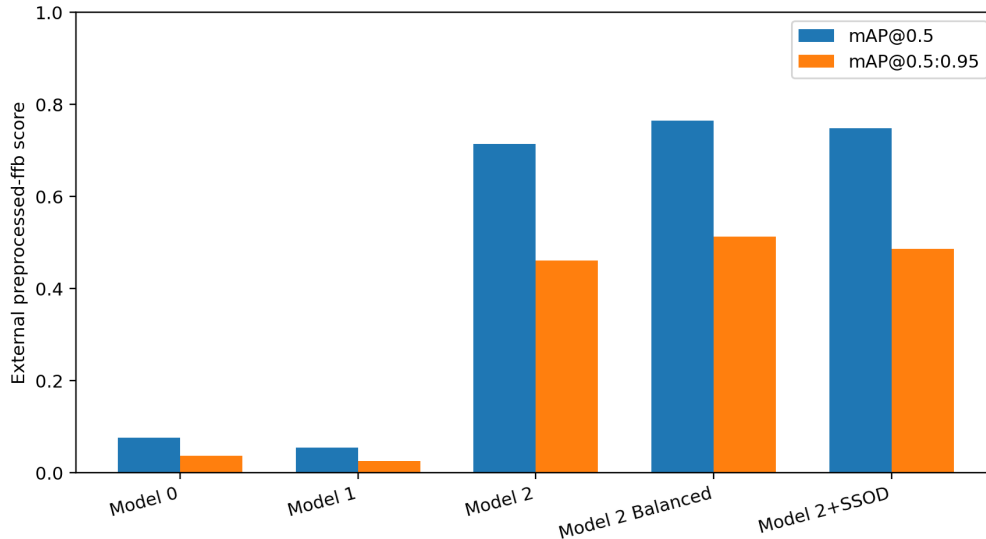
Figure 3: External-domain model comparison plot generated from the project reporting pipeline.
