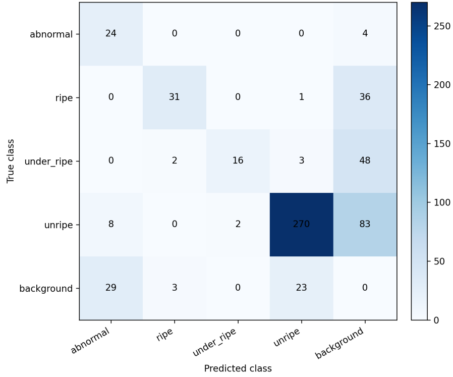
Figure 5: Locked external-domain confusion matrix for the strict SSOD model under the four-class masked protocol.
