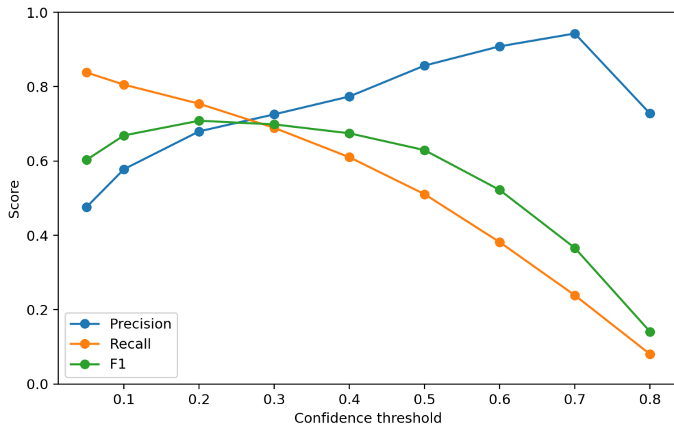
Figure 3: External-domain calibration curve used to select high-precision operating points.
