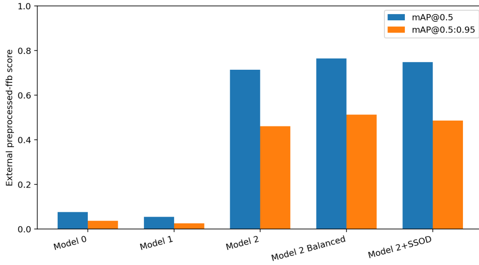
Figure 2: External-domain model comparison plot generated from the project reporting pipeline.
