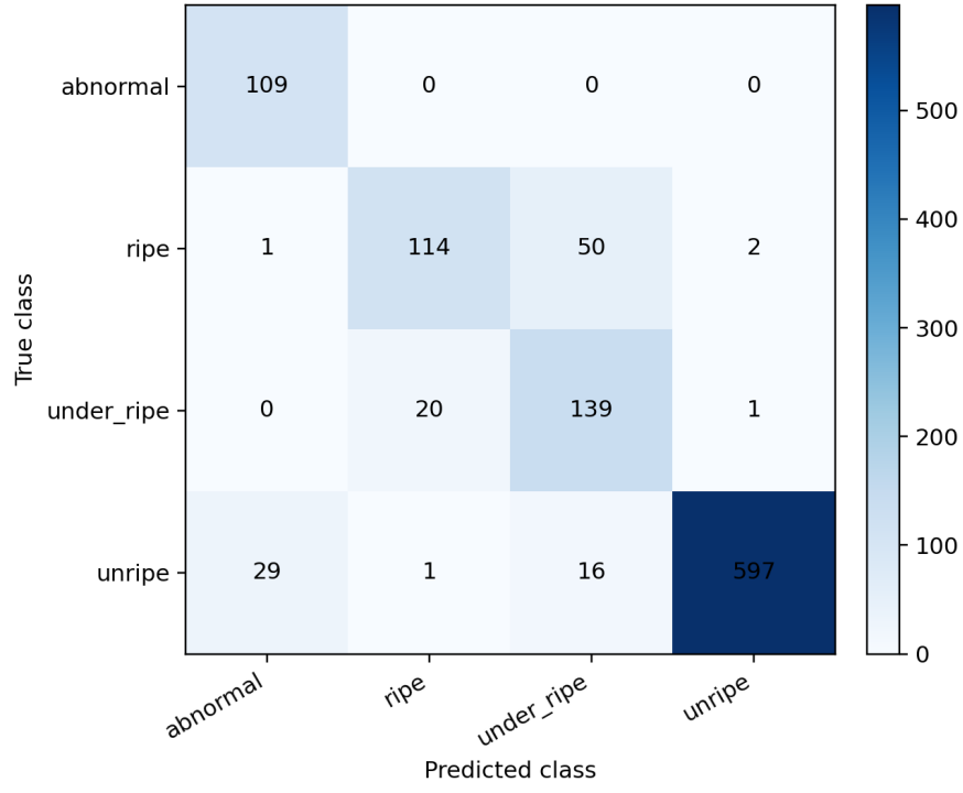
Figure 4: External-domain confusion matrix for the class-balanced target-domain adaptation model.
