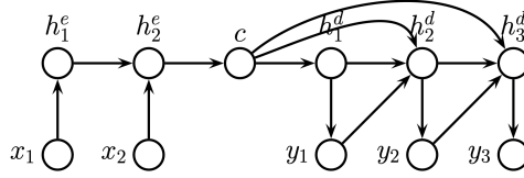
Figure 9: Encoder-decoder RNN architecture for mapping sequence \mathbf{x}_{1:T} to sequence \mathbf{y}_{1:T'}
