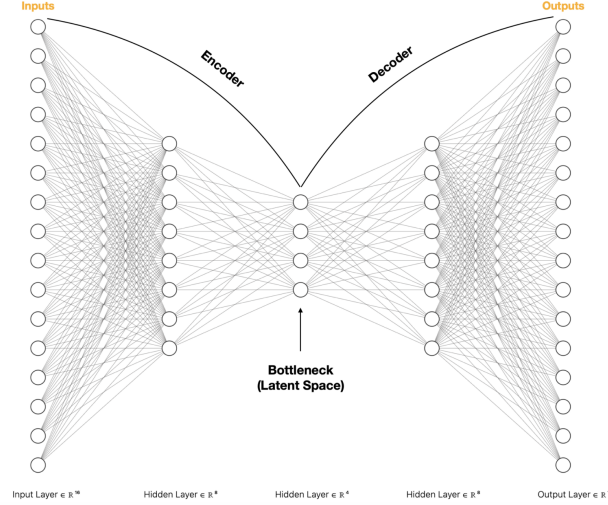
Figure 12: Schematic illustration of an undercomplete autoencoder.
