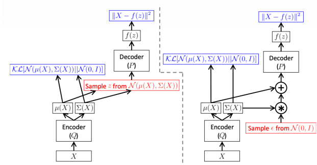
Figure 14: Computation graphs for VAEs. Computation graph for VAEs, where p(z) = \mathcal{N}(z|\mathbf{0}, \mathbf{I}) , p(x|z, \theta) = \mathcal{N}(x|f(z), \sigma^2 \mathbf{I}) , and q(z|x, \phi) = \mathcal{N}(z|\mu(x), \Sigma(x)) . Red boxes show sampling operations which are not differentiable. Blue boxes show loss layers (we assume Gaussian likelihoods and priors). (Left) Without the reparameterization trick. (Right) With the reparameterization trick. Gradients can flow from the output loss, back through the decoder and into the encoder.
