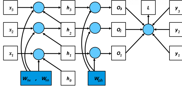
Figure 10: An RNN unrolled for 3 time steps, with the target output sequence and shown.
