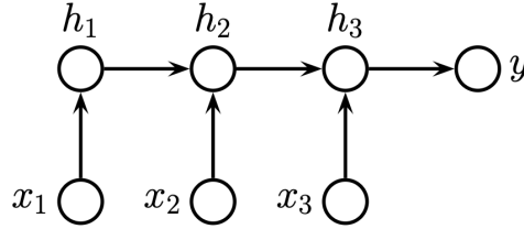
Figure 5: Simple Seq2Vec RNN for sequence classification.
