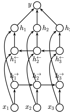
Figure 6: Bidirectional Seq2Vec RNN for sequence classification.
