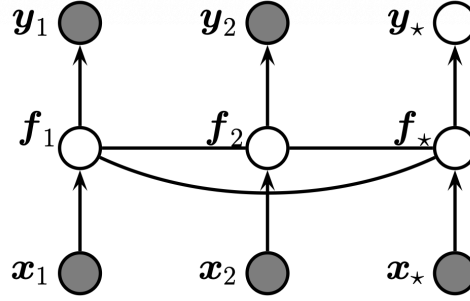
Figure 15: A Gaussian process for 2 training points and 1 test point. The hidden nodes f_i = f(\mathbf{x}_i) represent the value of the function at each of the data points. These hidden nodes are fully interconnected with the edge represent the covariance terms \Sigma_{ij} = \mathcal{K}(\mathbf{x}_i, \mathbf{x}_j) . If the testing points \mathbf{x}_* is close to the training points, then the predicted function value f(\mathbf{x}_*) will be similar to the training points f(\mathbf{x}_1) and f(\mathbf{x}_2) .
