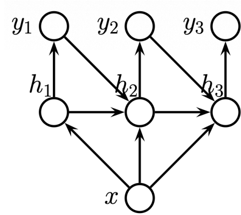
Figure 4: RNN for generating a variable length output sequence \mathbf{y}_{1:T} given an optional fixed length input vector \mathbf{x} .
