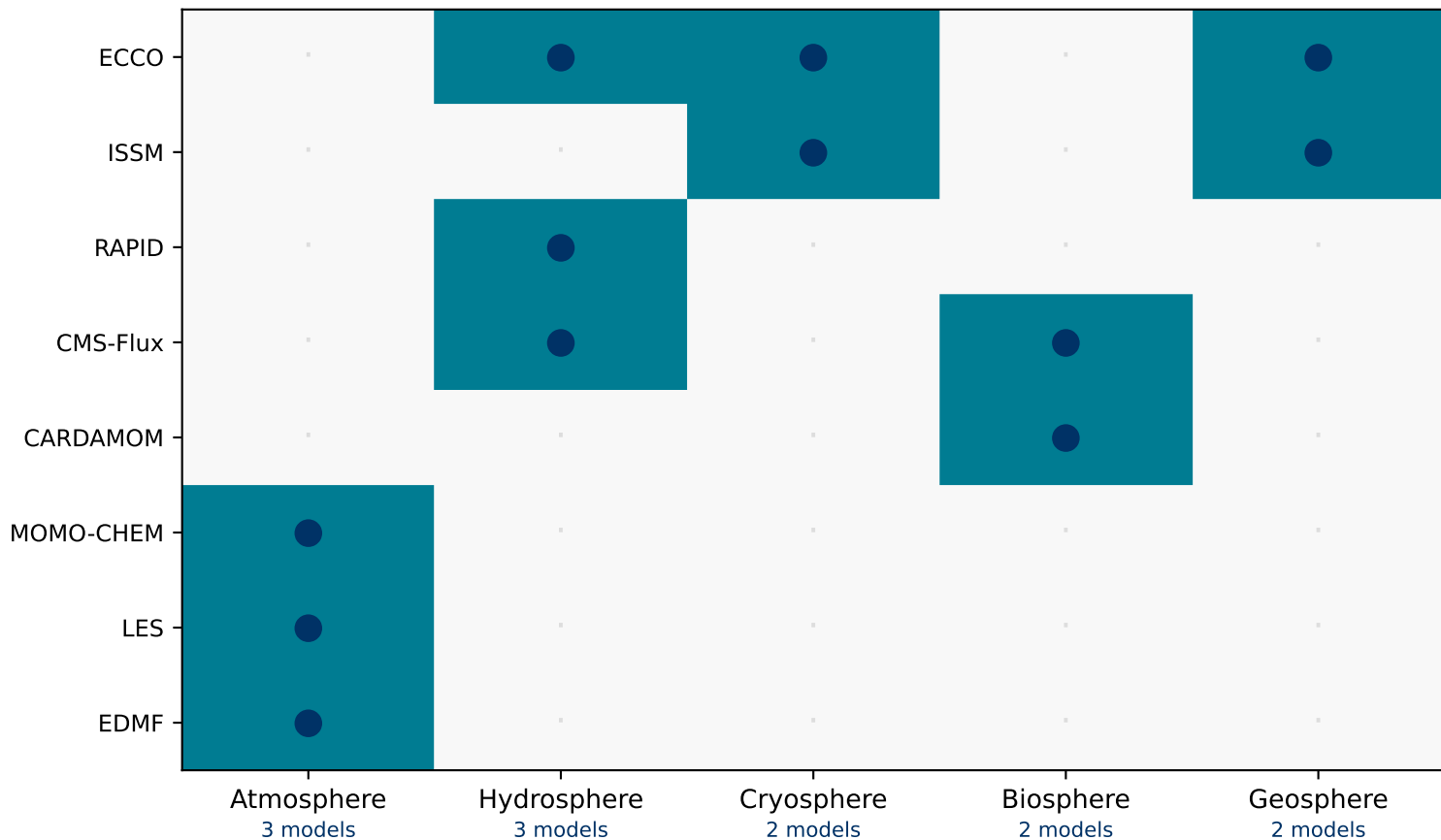
Figure 8. Model-to-Sphere Mapping: JEME Coverage of Earth System Components
