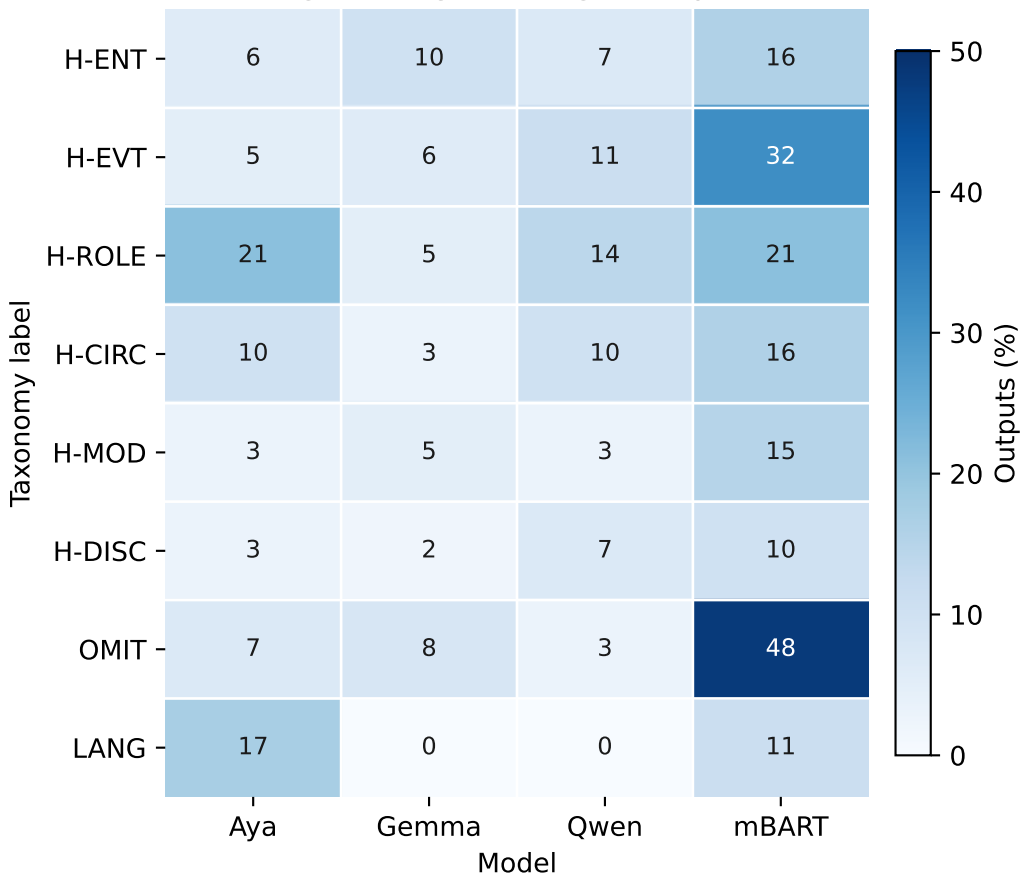
Fine-grained grounding-error profiles
