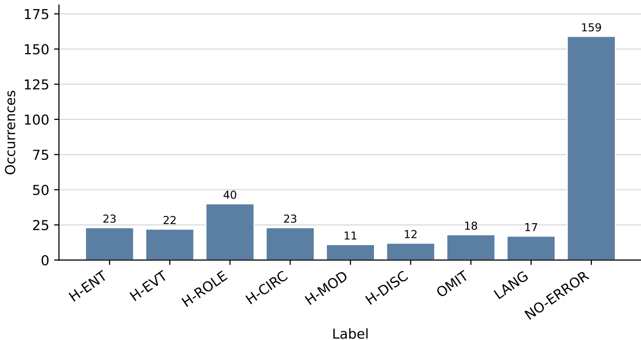
SLM taxonomy label counts
