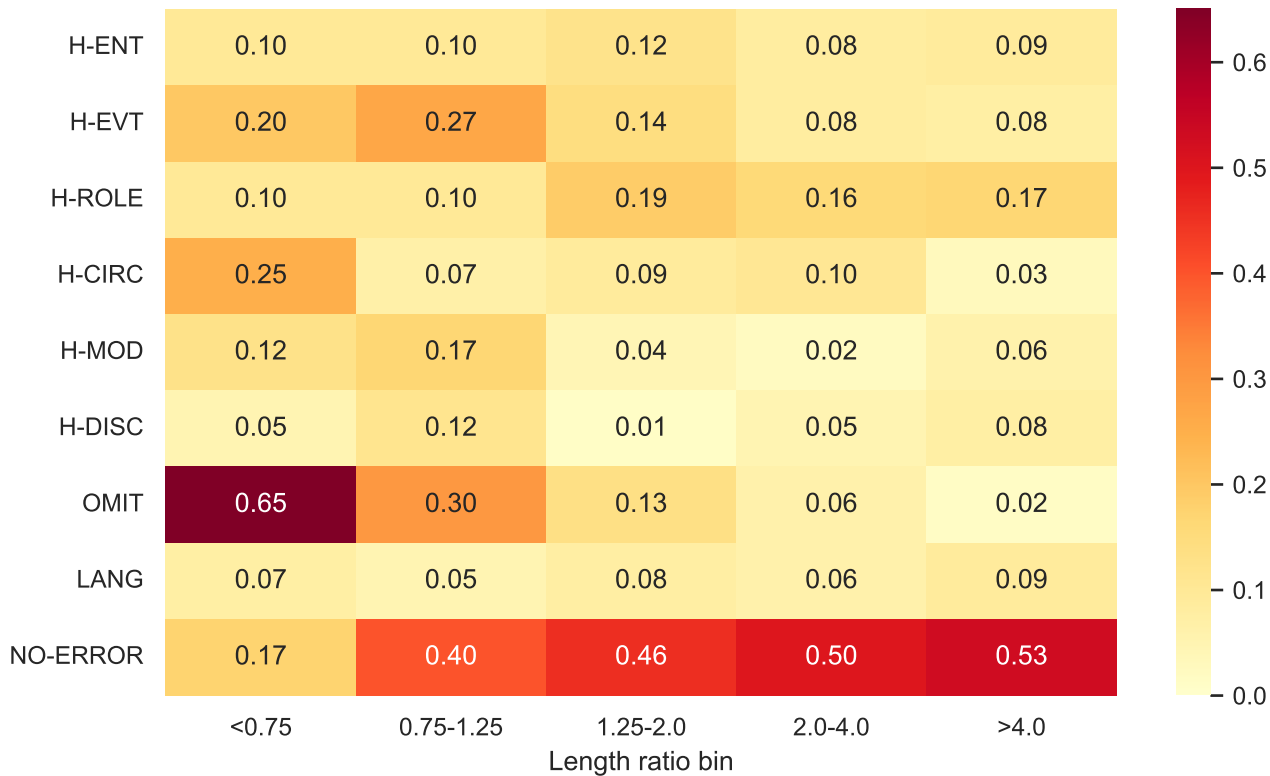
Label rates by length ratio bin
