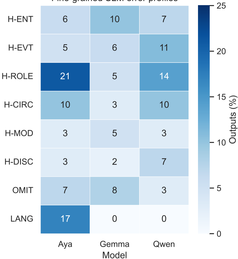
Fine-grained SLM error profiles
