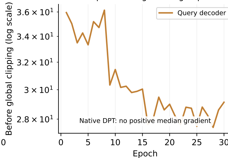
Median parameter-gradient group norm
